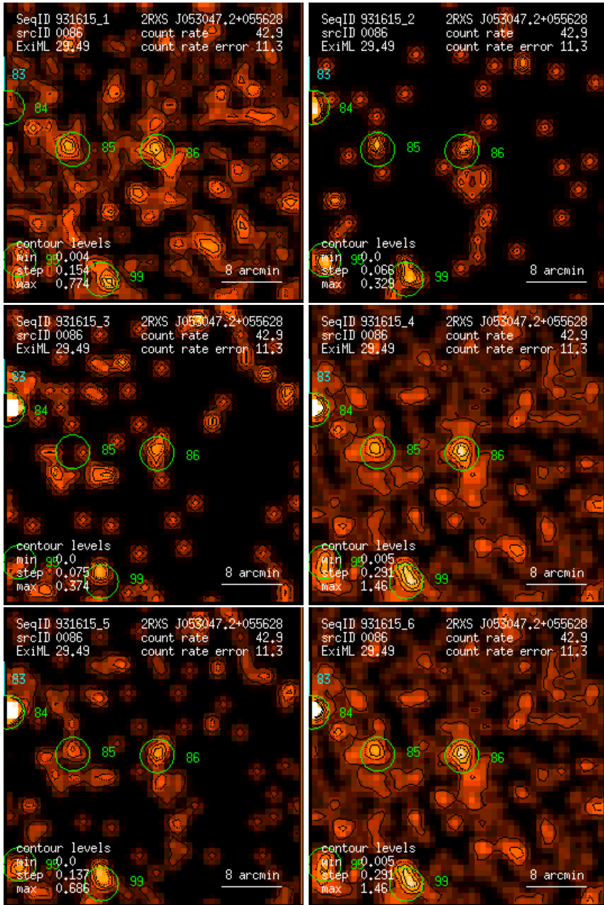
Figure 86: RASS 931615: detection 0086: band rate images, Gaussian filter: (1) PSPC channels 11 – 41, (2) 52 – 90, (3) 91 – 201, (4) 11 – 235, (5) 52 – 201, (6) 11 – 201. Broad band rates in counts/ks. Band rate contour levels in counts/ks/arcmin 2 .
