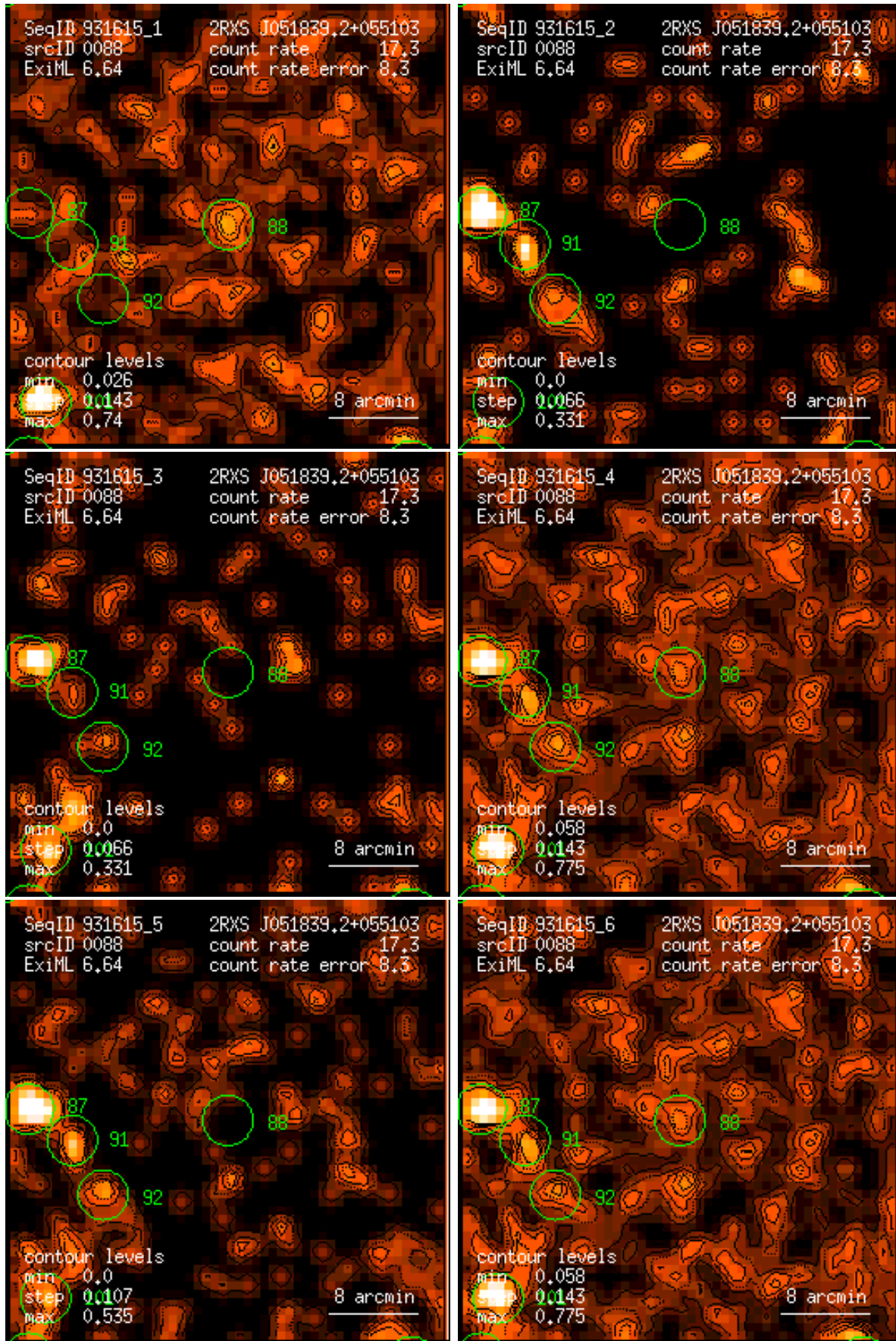
Figure 88: RASS 931615: detection 0088: band rate images, Gaussian filter: (1) PSPC channels 11 – 41, (2) 52 – 90, (3) 91 – 201, (4) 11 – 235, (5) 52 – 201, (6) 11 – 201. Broad band rates in counts/ks. Band rate contour levels in counts/ks/arcmin 2 .
