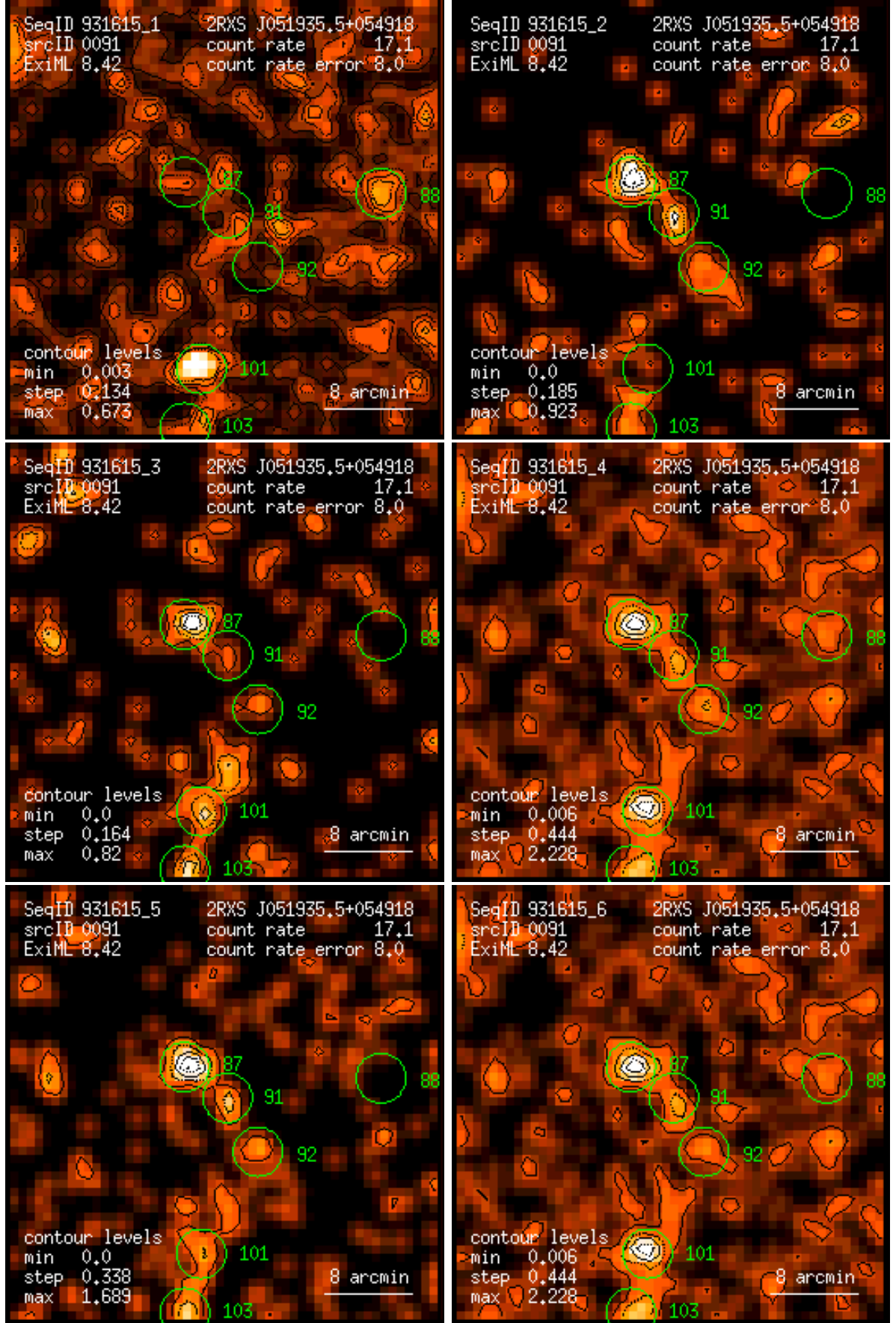
Figure 91: RASS 931615: detection 0091: band rate images, Gaussian filter: (1) PSPC channels 11 – 41, (2) 52 – 90, (3) 91 – 201, (4) 11 – 235, (5) 52 – 201, (6) 11 – 201. Broad band rates in counts/ks. Band rate contour levels in counts/ks/arcmin 2 .
