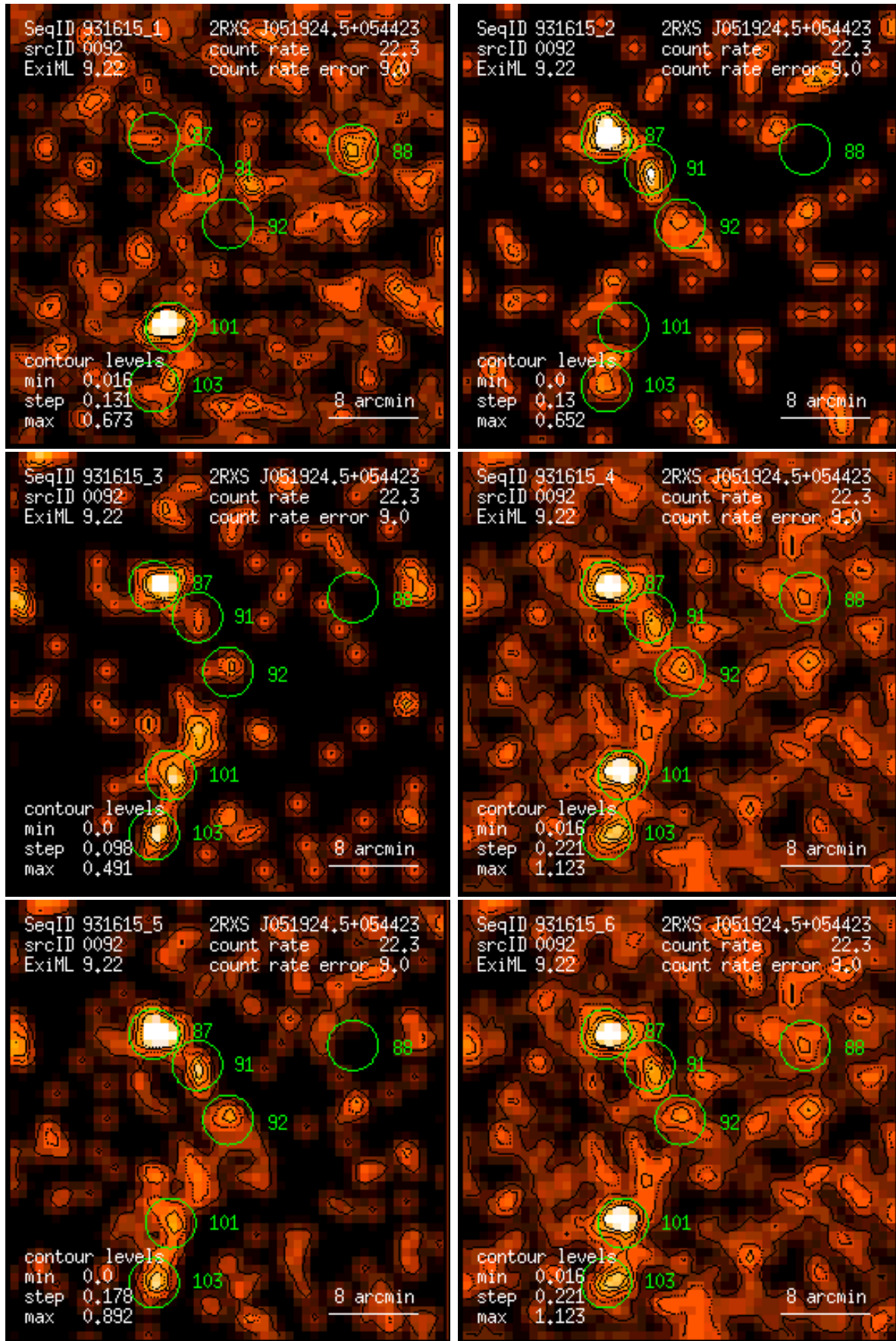
Figure 92: RASS 931615: detection 0092: band rate images, Gaussian filter: (1) PSPC channels 11 – 41, (2) 52 – 90, (3) 91 – 201, (4) 11 – 235, (5) 52 – 201, (6) 11 – 201. Broad band rates in counts/ks. Band rate contour levels in counts/ks/arcmin 2 .
