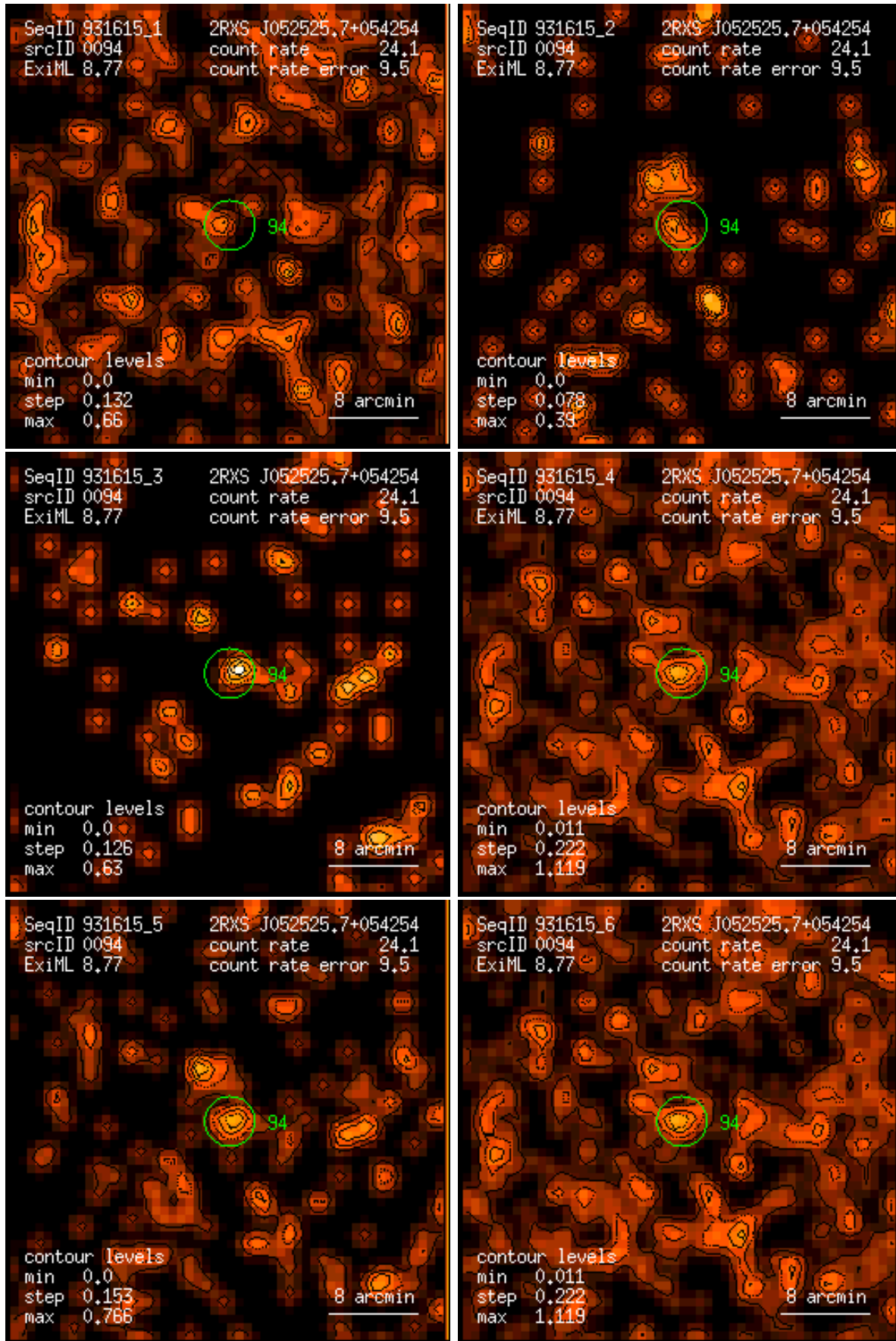
Figure 94: RASS 931615: detection 0094: band rate images, Gaussian filter: (1) PSPC channels 11 – 41, (2) 52 – 90, (3) 91 – 201, (4) 11 – 235, (5) 52 – 201, (6) 11 – 201. Broad band rates in counts/ks. Band rate contour levels in counts/ks/arcmin 2 .
