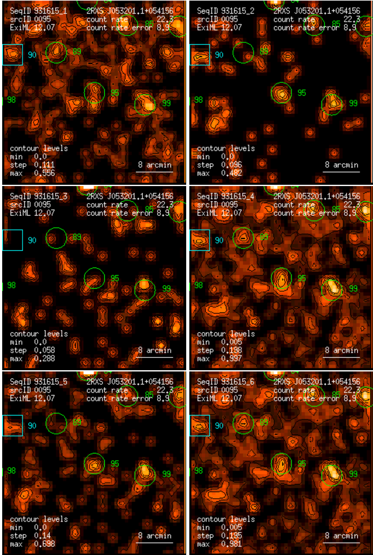
Figure 95: RASS 931615: detection 0095: band rate images, Gaussian filter: (1) PSPC channels 11 – 41, (2) 52 – 90, (3) 91 – 201, (4) 11 – 235, (5) 52 – 201, (6) 11 – 201. Broad band rates in counts/ks. Band rate contour levels in counts/ks/arcmin 2 .
