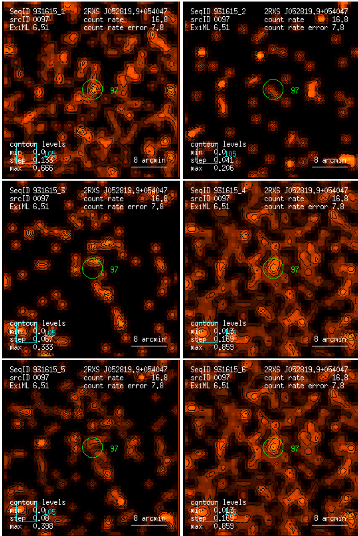
Figure 97: RASS 931615: detection 0097: band rate images, Gaussian filter: (1) PSPC channels 11 – 41, (2) 52 – 90, (3) 91 – 201, (4) 11 – 235, (5) 52 – 201, (6) 11 – 201. Broad band rates in counts/ks. Band rate contour levels in counts/ks/arcmin 2 .
