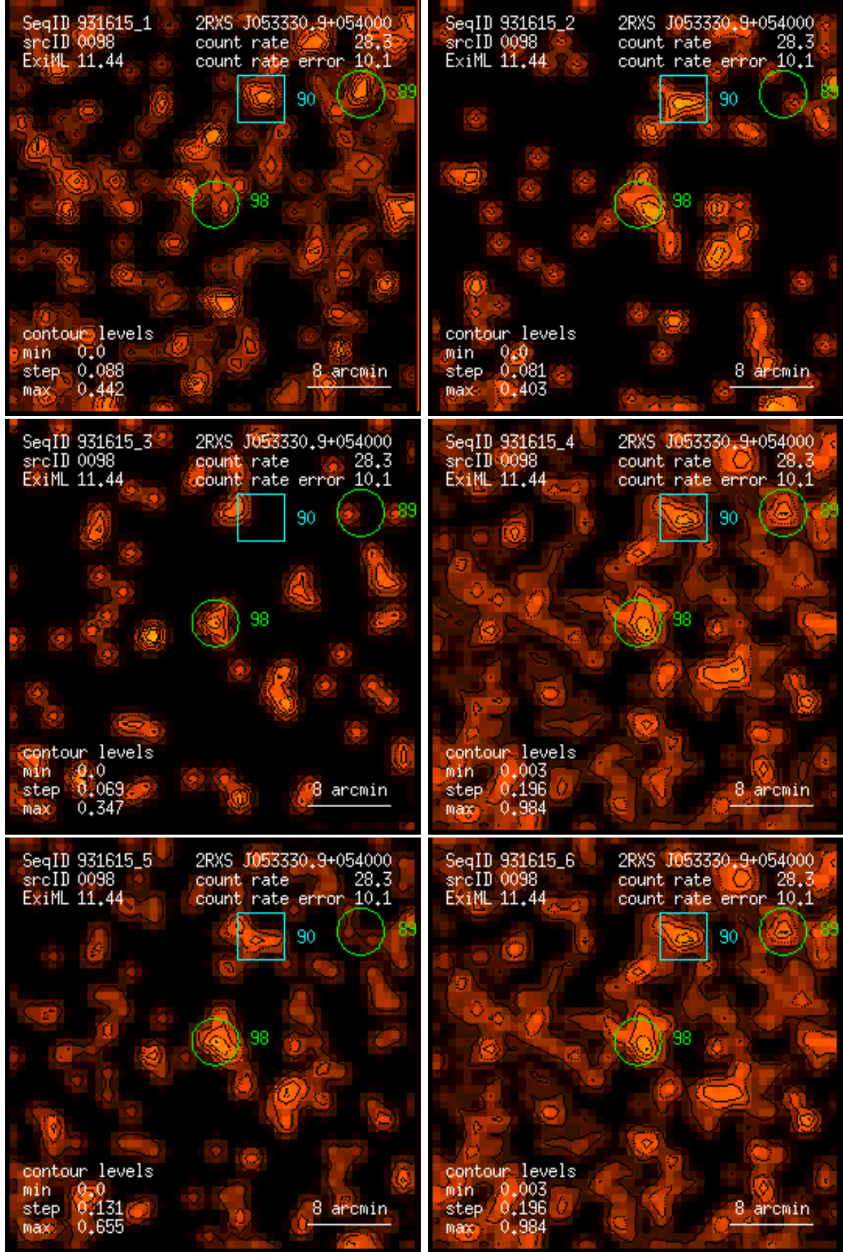
Figure 98: RASS 931615: detection 0098: band rate images, Gaussian filter: (1) PSPC channels 11 – 41, (2) 52 – 90, (3) 91 – 201, (4) 11 – 235, (5) 52 – 201, (6) 11 – 201. Broad band rates in counts/ks. Band rate contour levels in counts/ks/arcmin 2 .
