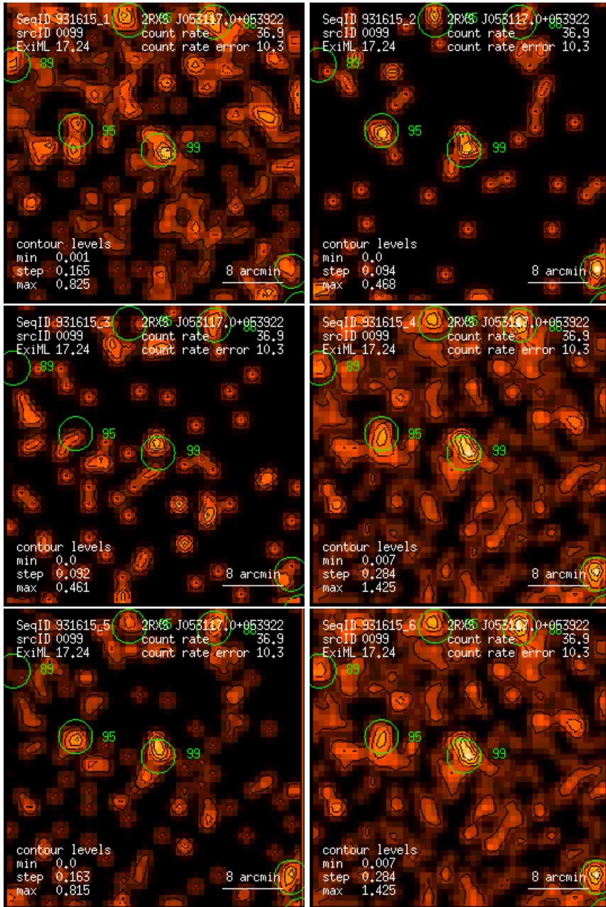
Figure 99: RASS 931615: detection 0099: band rate images, Gaussian filter: (1) PSPC channels 11 – 41, (2) 52 – 90, (3) 91 – 201, (4) 11 – 235, (5) 52 – 201, (6) 11 – 201. Broad band rates in counts/ks. Band rate contour levels in counts/ks/arcmin 2 .
