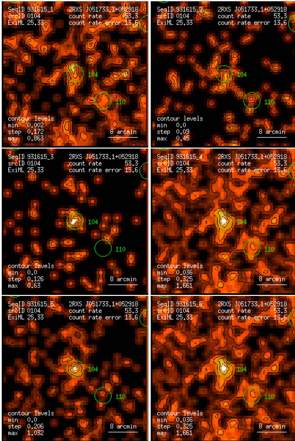
Figure 104: RASS 931615: detection 0104: band rate images, Gaussian filter: (1) PSPC channels 11 – 41, (2) 52 – 90, (3) 91 – 201, (4) 11 – 235, (5) 52 – 201, (6) 11 – 201. Broad band rates in counts/ks. Band rate contour levels in counts/ks/arcmin 2 .
