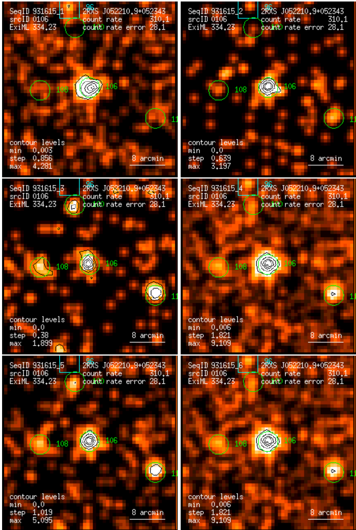
Figure 106: RASS 931615: detection 0106: band rate images, Gaussian filter: (1) PSPC channels 11 – 41, (2) 52 – 90, (3) 91 – 201, (4) 11 – 235, (5) 52 – 201, (6) 11 – 201. Broad band rates in counts/ks. Band rate contour levels in counts/ks/arcmin 2 .
