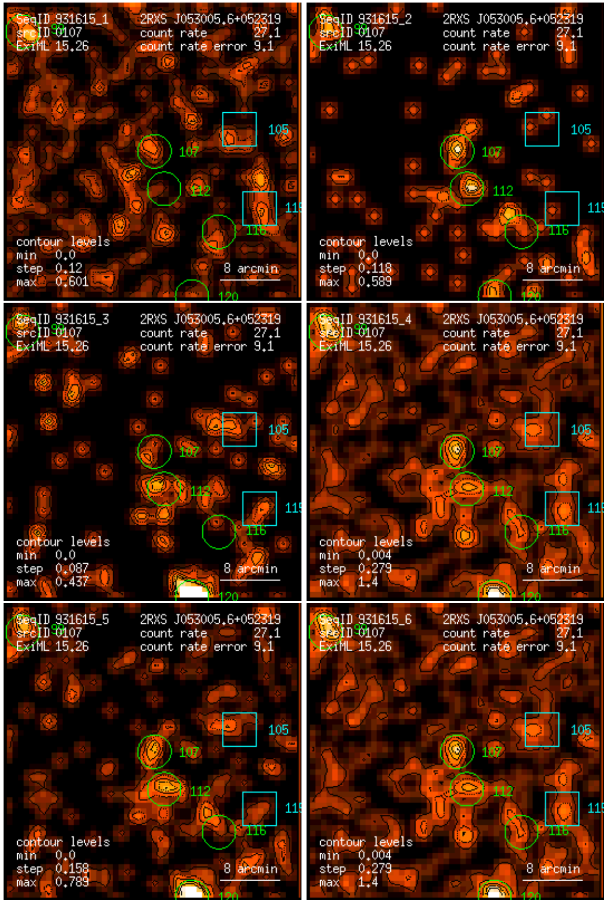
Figure 107: RASS 931615: detection 0107: band rate images, Gaussian filter: (1) PSPC channels 11 – 41, (2) 52 – 90, (3) 91 – 201, (4) 11 – 235, (5) 52 – 201, (6) 11 – 201. Broad band rates in counts/ks. Band rate contour levels in counts/ks/arcmin 2 .
