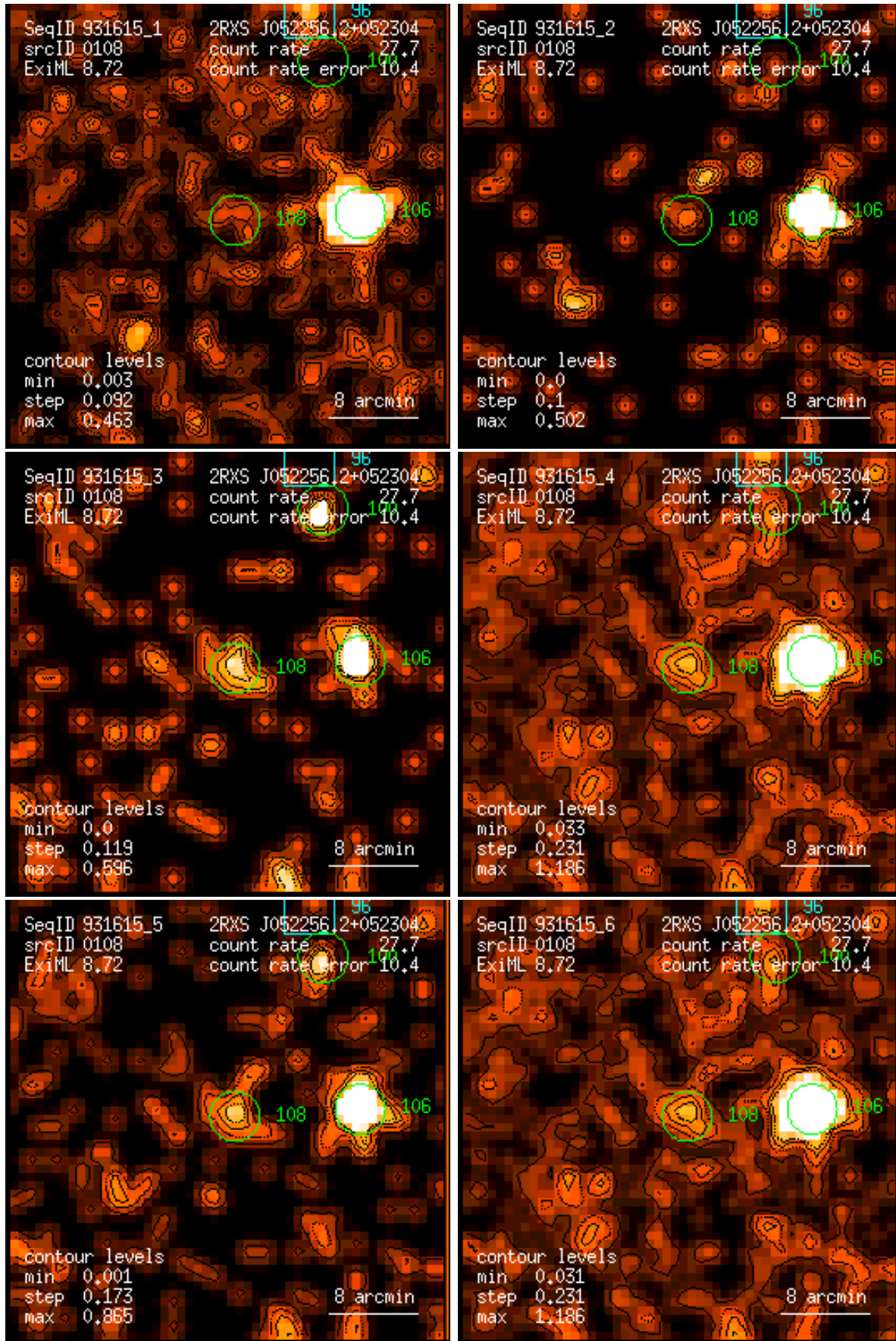
Figure 108: RASS 931615: detection 0108: band rate images, Gaussian filter: (1) PSPC channels 11 – 41, (2) 52 – 90, (3) 91 – 201, (4) 11 – 235, (5) 52 – 201, (6) 11 – 201. Broad band rates in counts/ks. Band rate contour levels in counts/ks/arcmin 2 .
