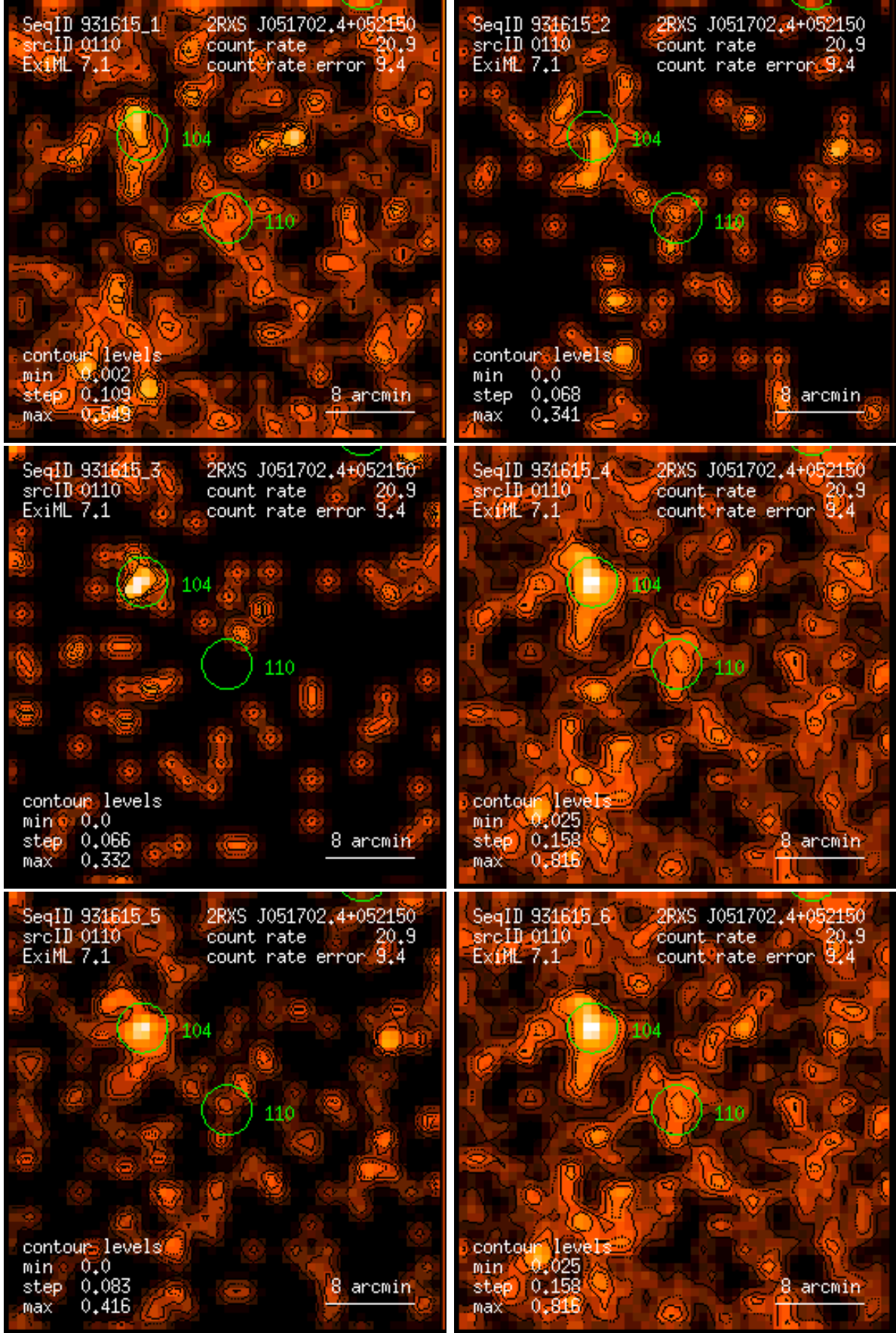
Figure 110: RASS 931615: detection 0110: band rate images, Gaussian filter: (1) PSPC channels 11 – 41, (2) 52 – 90, (3) 91 – 201, (4) 11 – 235, (5) 52 – 201, (6) 11 – 201. Broad band rates in counts/ks. Band rate contour levels in counts/ks/arcmin 2 .
