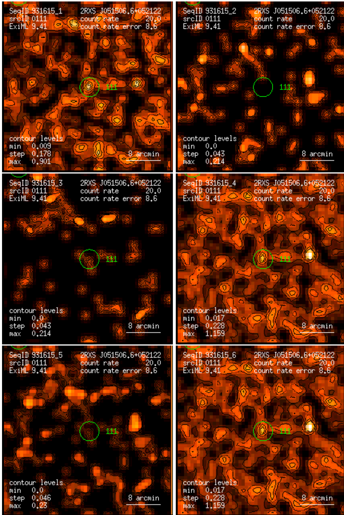
Figure 111: RASS 931615: detection 0111: band rate images, Gaussian filter: (1) PSPC channels 11 – 41, (2) 52 – 90, (3) 91 – 201, (4) 11 – 235, (5) 52 – 201, (6) 11 – 201. Broad band rates in counts/ks. Band rate contour levels in counts/ks/arcmin 2 .
