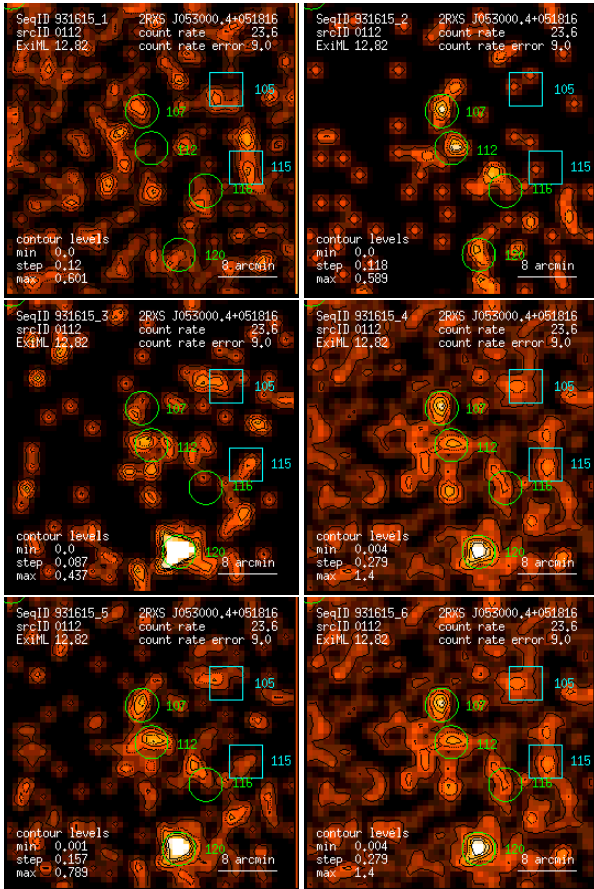
Figure 112: RASS 931615: detection 0112: band rate images, Gaussian filter: (1) PSPP channels 11 – 41, (2) 52 – 90, (3) 91 – 201, (4) 11 – 235, (5) 52 – 201, (6) 11 – 201. Broad band rates in counts/ks. Band rate contour levels in counts/ks/arcmin 2 .
