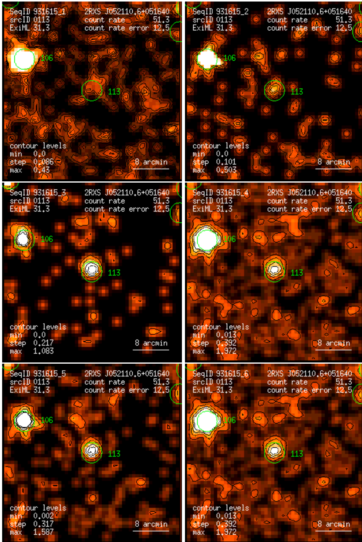
Figure 113: RASS 931615: detection 0113: band rate images, Gaussian filter: (1) PSPC channels 11 – 41, (2) 52 – 90, (3) 91 – 201, (4) 11 – 235, (5) 52 – 201, (6) 11 – 201. Broad band rates in counts/ks. Band rate contour levels in counts/ks/arcmin 2 .
