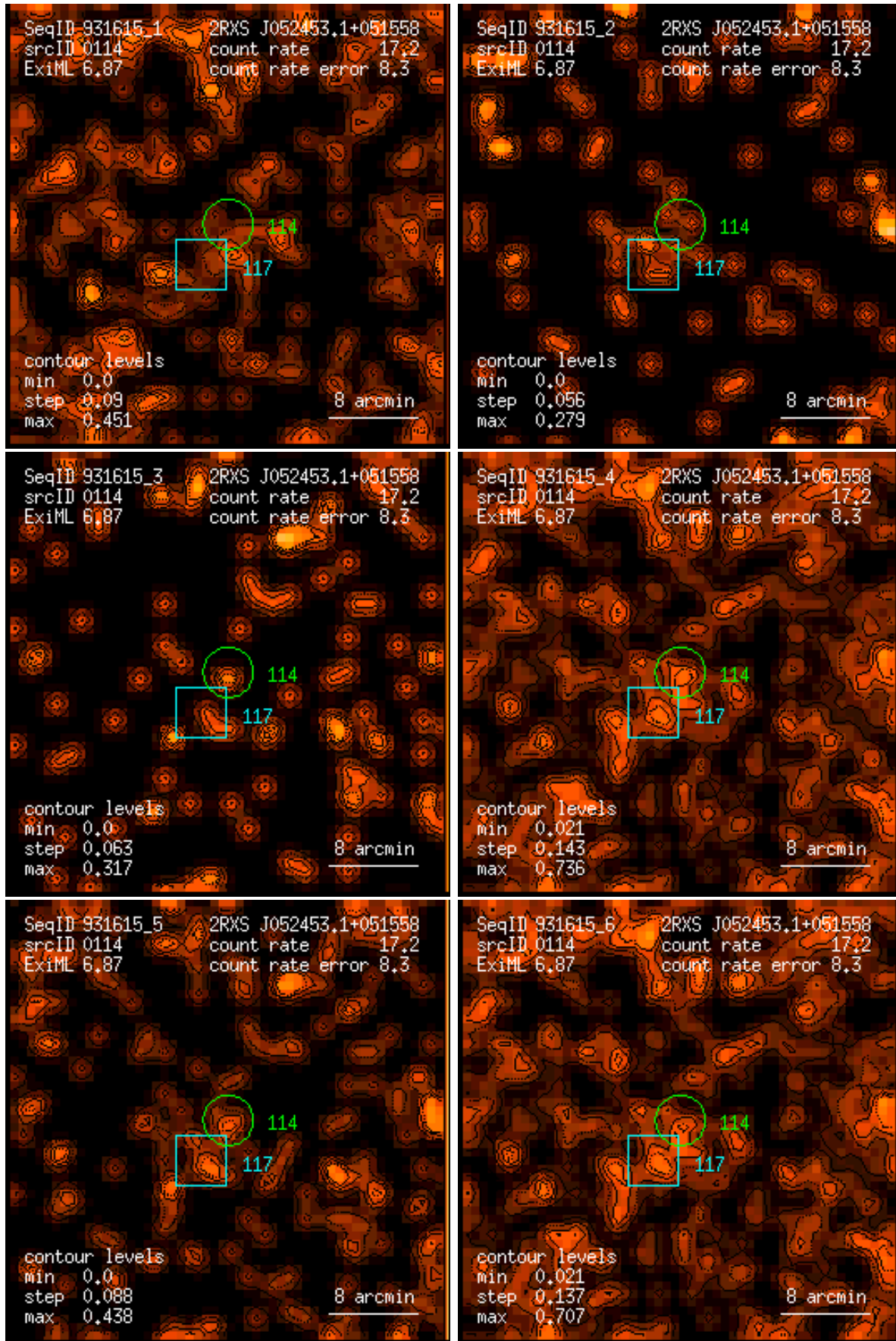
Figure 114: RASS 931615: detection 0114: band rate images, Gaussian filter: (1) PSPC channels 11 – 41, (2) 52 – 90, (3) 91 – 201, (4) 11 – 235, (5) 52 – 201, (6) 11 – 201. Broad band rates in counts/ks. Band rate contour levels in counts/ks/arcmin 2 .
