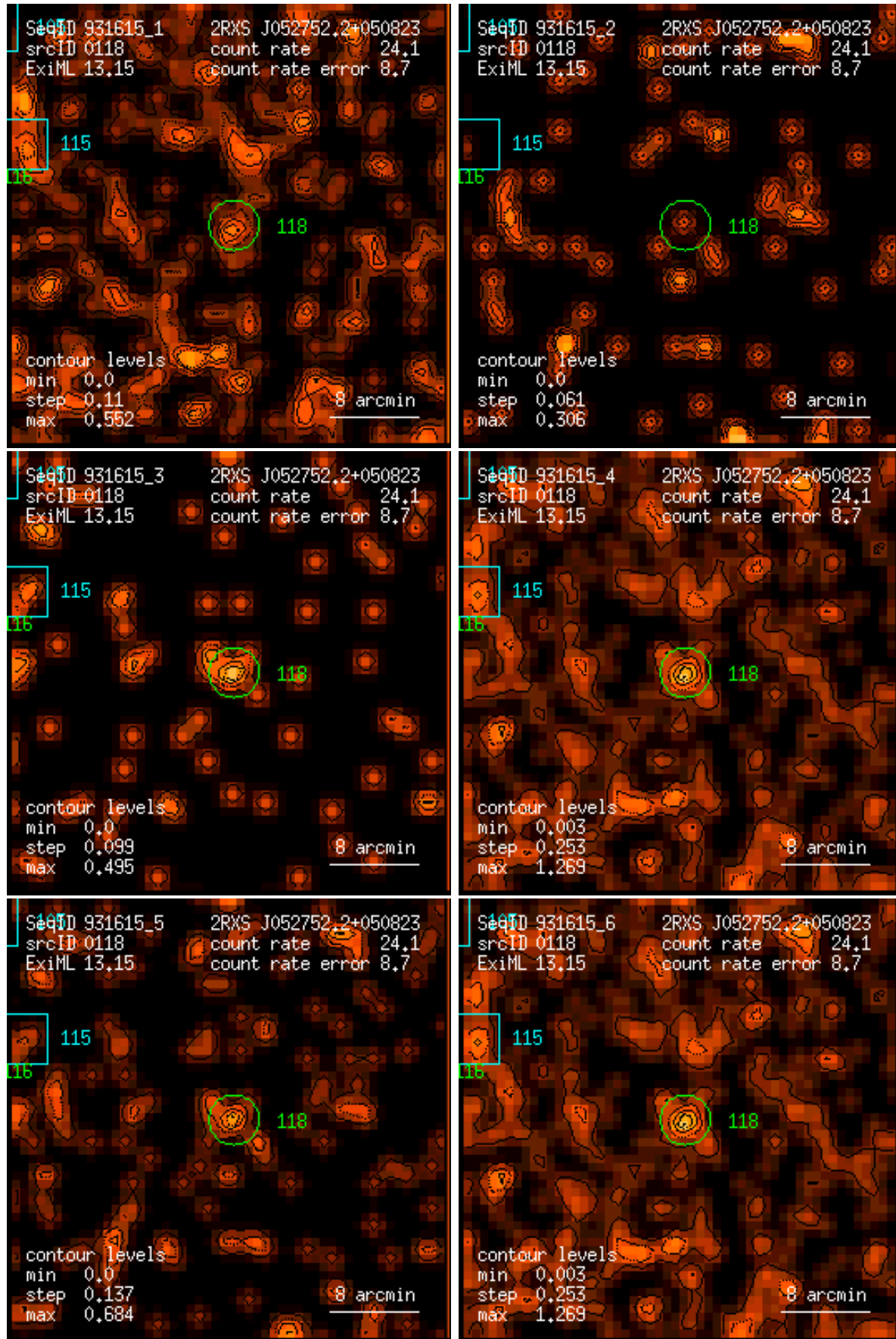
Figure 118: RASS 931615: detection 0118: band rate images, Gaussian filter: (1) PSPC channels 11 – 41, (2) 52 – 90, (3) 91 – 201, (4) 11 – 235, (5) 52 – 201, (6) 11 – 201. Broad band rates in counts/ks. Band rate contour levels in counts/ks/arcmin 2 .
