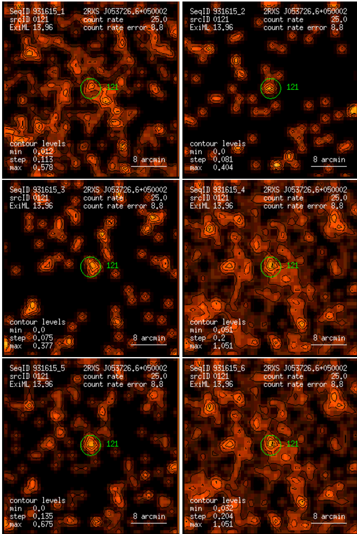
Figure 121: RASS 931615: detection 0121: band rate images, Gaussian filter: (1) PSPC channels 11 – 41, (2) 52 – 90, (3) 91 – 201, (4) 11 – 235, (5) 52 – 201, (6) 11 – 201. Broad band rates in counts/ks. Band rate contour levels in counts/ks/arcmin 2 .
