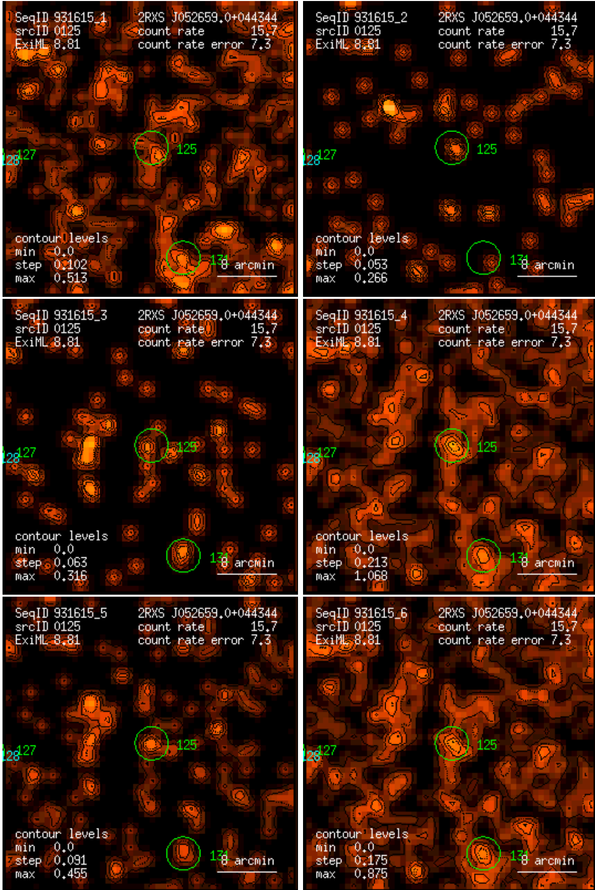
Figure 125: RASS 931615: detection 0125: band rate images, Gaussian filter: (1) PSPC channels 11 – 41, (2) 52 – 90, (3) 91 – 201, (4) 11 – 235, (5) 52 – 201, (6) 11 – 201. Broad band rates in counts/ks. Band rate contour levels in counts/ks/arcmin 2 .
