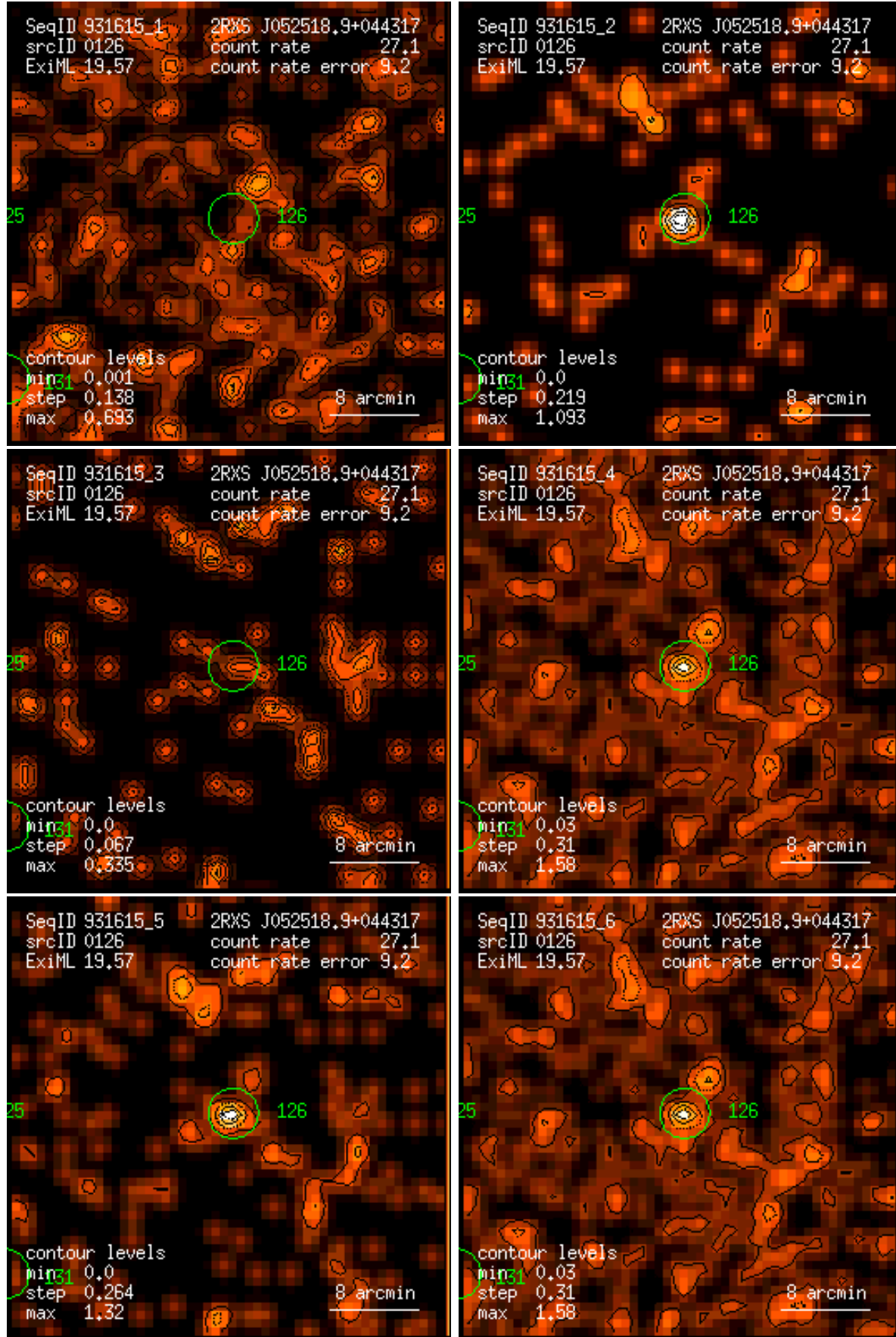
Figure 126: RASS 931615: detection 0126: band rate images, Gaussian filter: (1) PSPC channels 11 – 41, (2) 52 – 90, (3) 91 – 201, (4) 11 – 235, (5) 52 – 201, (6) 11 – 201. Broad band rates in counts/ks. Band rate contour levels in counts/ks/arcmin 2 .
