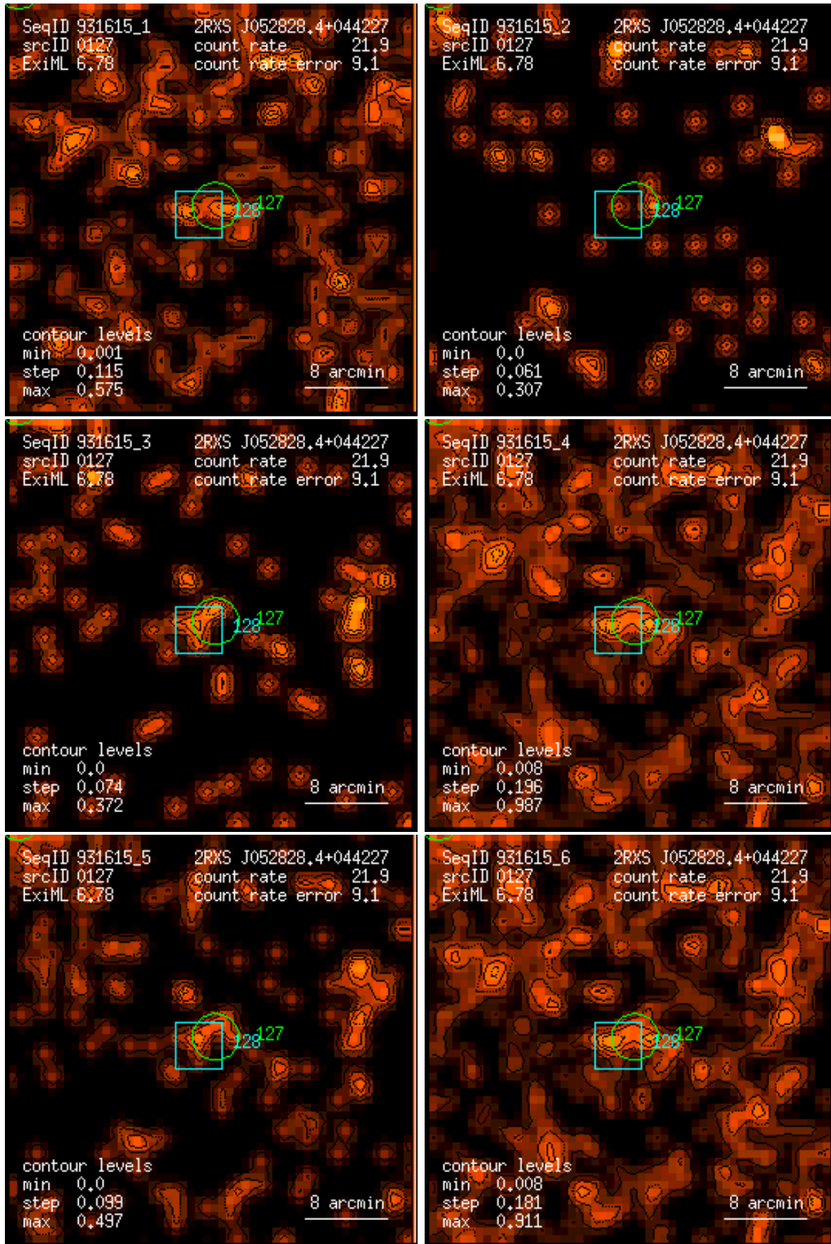
Figure 127: RASS 931615: detection 0127: band rate images, Gaussian filter: (1) PSPC channels 11 – 41, (2) 52 – 90, (3) 91 – 201, (4) 11 – 235, (5) 52 – 201, (6) 11 – 201. Broad band rates in counts/ks. Band rate contour levels in counts/ks/arcmin 2 .
