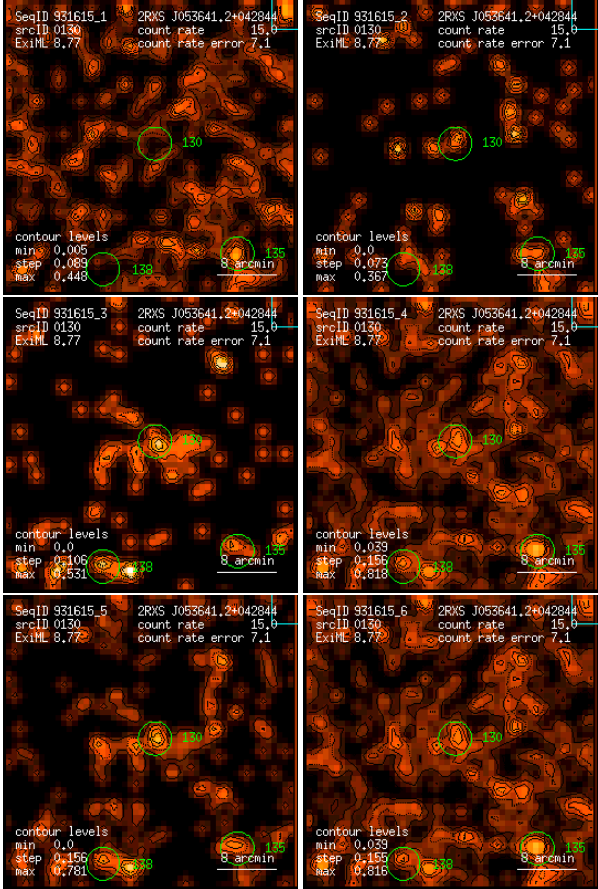
Figure 130: RASS 931615: detection 0130: band rate images, Gaussian filter: (1) PSPC channels 11 – 41, (2) 52 – 90, (3) 91 – 201, (4) 11 – 235, (5) 52 – 201, (6) 11 – 201. Broad band rates in counts/ks. Band rate contour levels in counts/ks/arcmin 2 .
