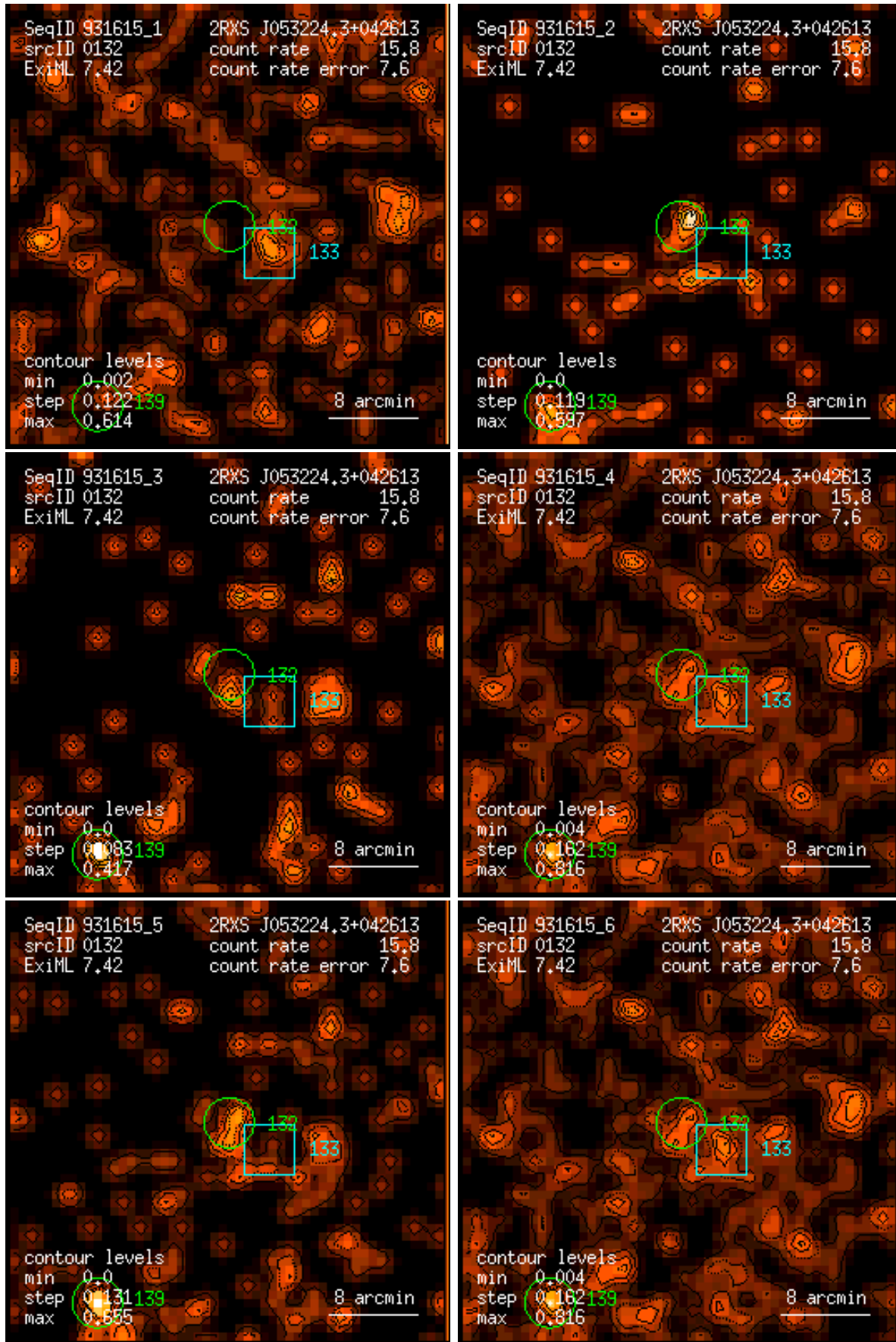
Figure 132: RASS 931615: detection 0132: band rate images, Gaussian filter: (1) PSPC channels 11 – 41, (2) 52 – 90, (3) 91 – 201, (4) 11 – 235, (5) 52 – 201, (6) 11 – 201. Broad band rates in counts/ks. Band rate contour levels in counts/ks/arcmin 2 .
