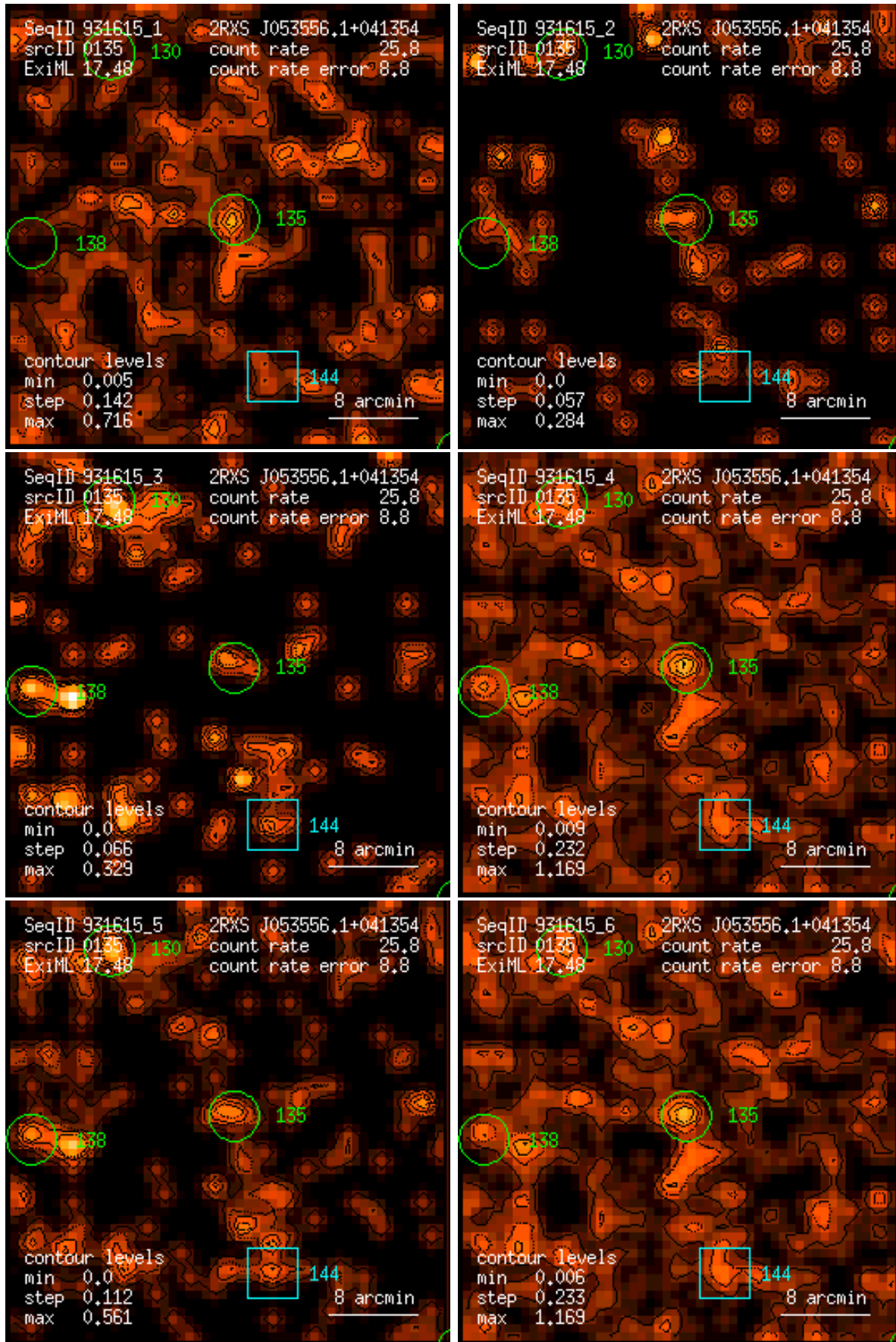
Figure 135: RASS 931615: detection 0135: band rate images, Gaussian filter: (1) PSPC channels 11 – 41, (2) 52 – 90, (3) 91 – 201, (4) 11 – 235, (5) 52 – 201, (6) 11 – 201. Broad band rates in counts/ks. Band rate contour levels in counts/ks/arcmin 2 .
