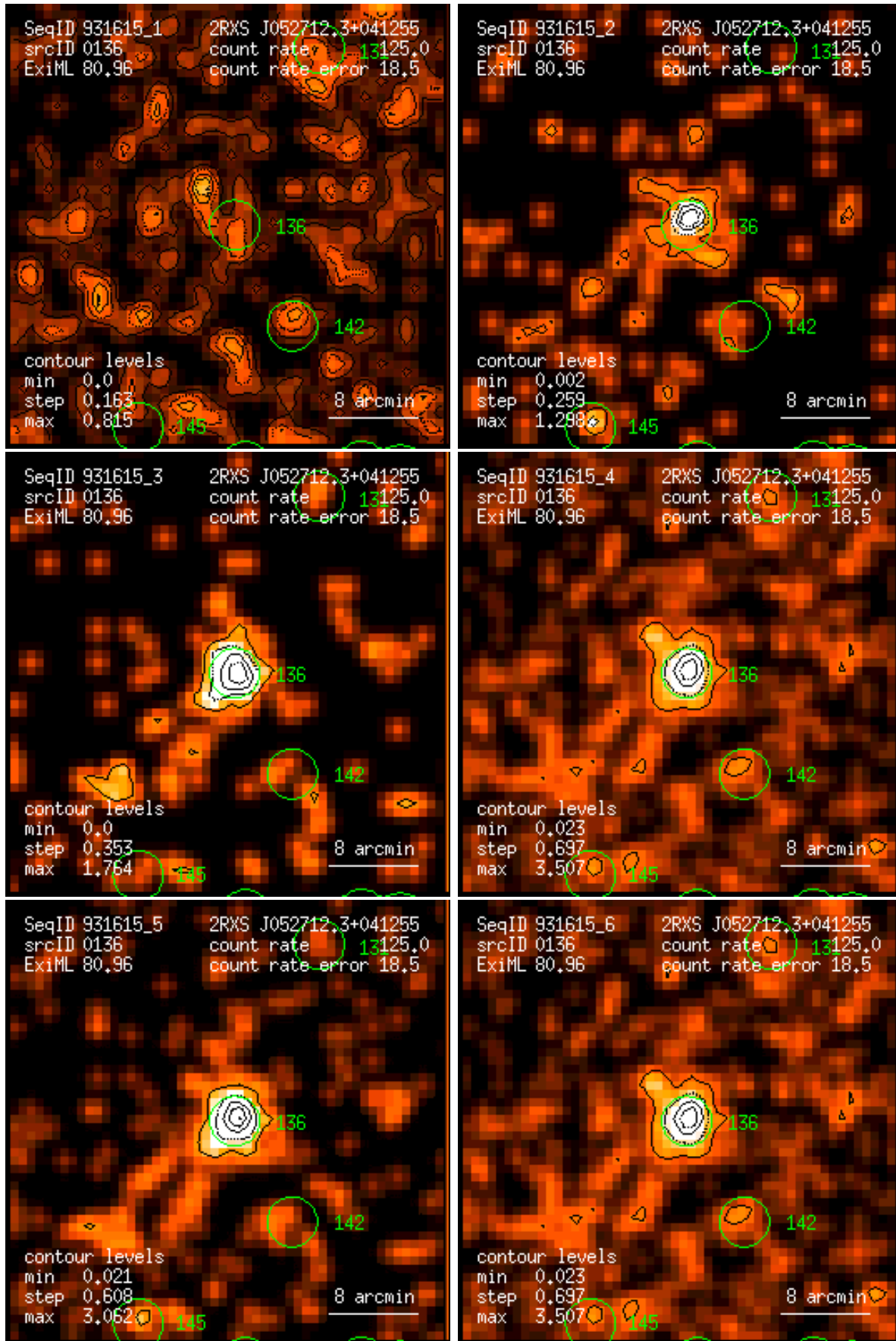
Figure 136: RASS 931615: detection 0136: band rate images, Gaussian filter: (1) PSPC channels 11 – 41, (2) 52 – 90, (3) 91 – 201, (4) 11 – 235, (5) 52 – 201, (6) 11 – 201. Broad band rates in counts/ks. Band rate contour levels in counts/ks/arcmin 2 .
