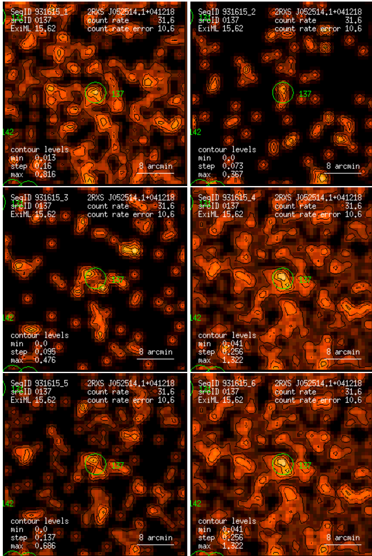
Figure 137: RASS 931615: detection 0137: band rate images, Gaussian filter: (1) PSPC channels 11 – 41, (2) 52 – 90, (3) 91 – 201, (4) 11 – 235, (5) 52 – 201, (6) 11 – 201. Broad band rates in counts/ks. Band rate contour levels in counts/ks/arcmin 2 .
