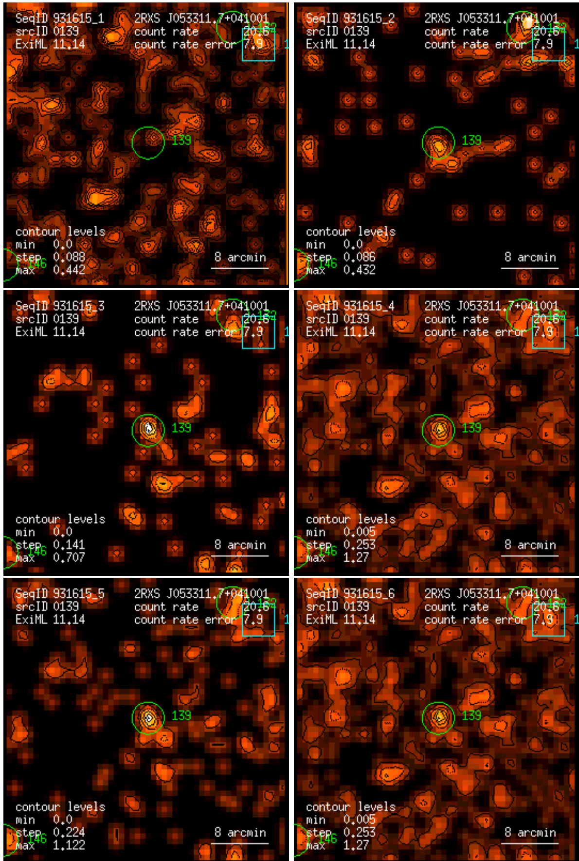
Figure 139: RASS 931615: detection 0139: band rate images, Gaussian filter: (1) PSPC channels 11 – 41, (2) 52 – 90, (3) 91 – 201, (4) 11 – 235, (5) 52 – 201, (6) 11 – 201. Broad band rates in counts/ks. Band rate contour levels in counts/ks/arcmin 2 .
