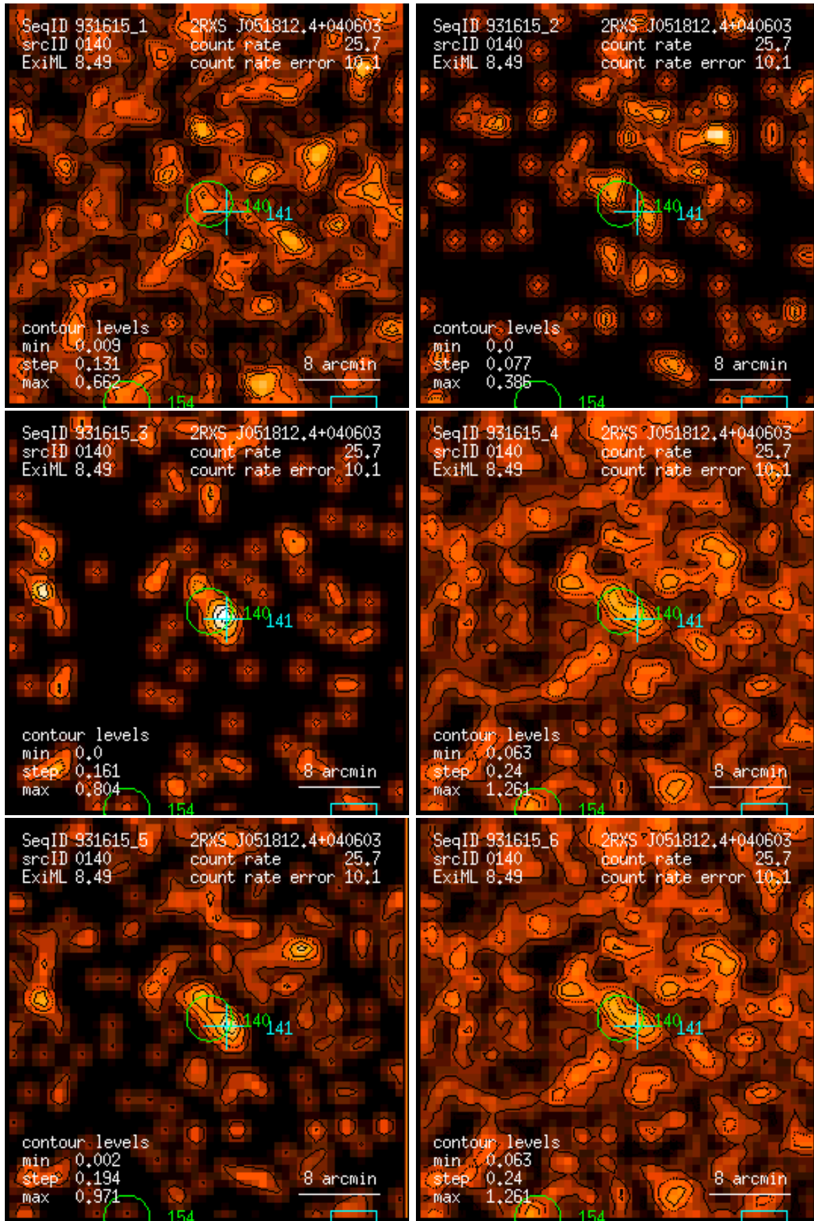
Figure 140: RASS 931615: detection 0140: band rate images, Gaussian filter: (1) PSPC channels 11 – 41, (2) 52 – 90, (3) 91 – 201, (4) 11 – 235, (5) 52 – 201, (6) 11 – 201. Broad band rates in counts/ks. Band rate contour levels in counts/ks/arcmin 2 .
