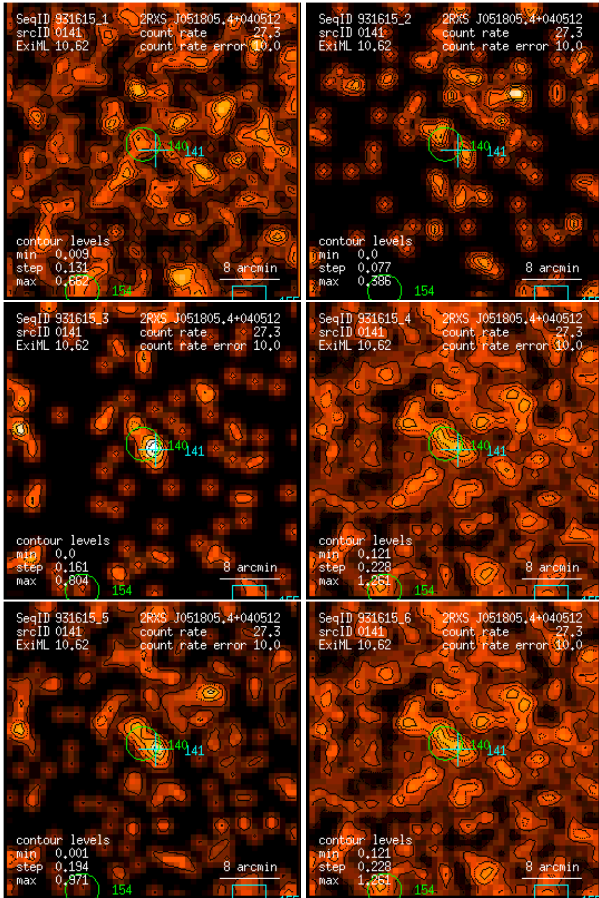
Figure 141: RASS 931615: detection 0141: band rate images, Gaussian filter: (1) PSPC channels 11 – 41, (2) 52 – 90, (3) 91 – 201, (4) 11 – 235, (5) 52 – 201, (6) 11 – 201. Broad band rates in counts/ks. Band rate contour levels in counts/ks/arcmin 2 .
