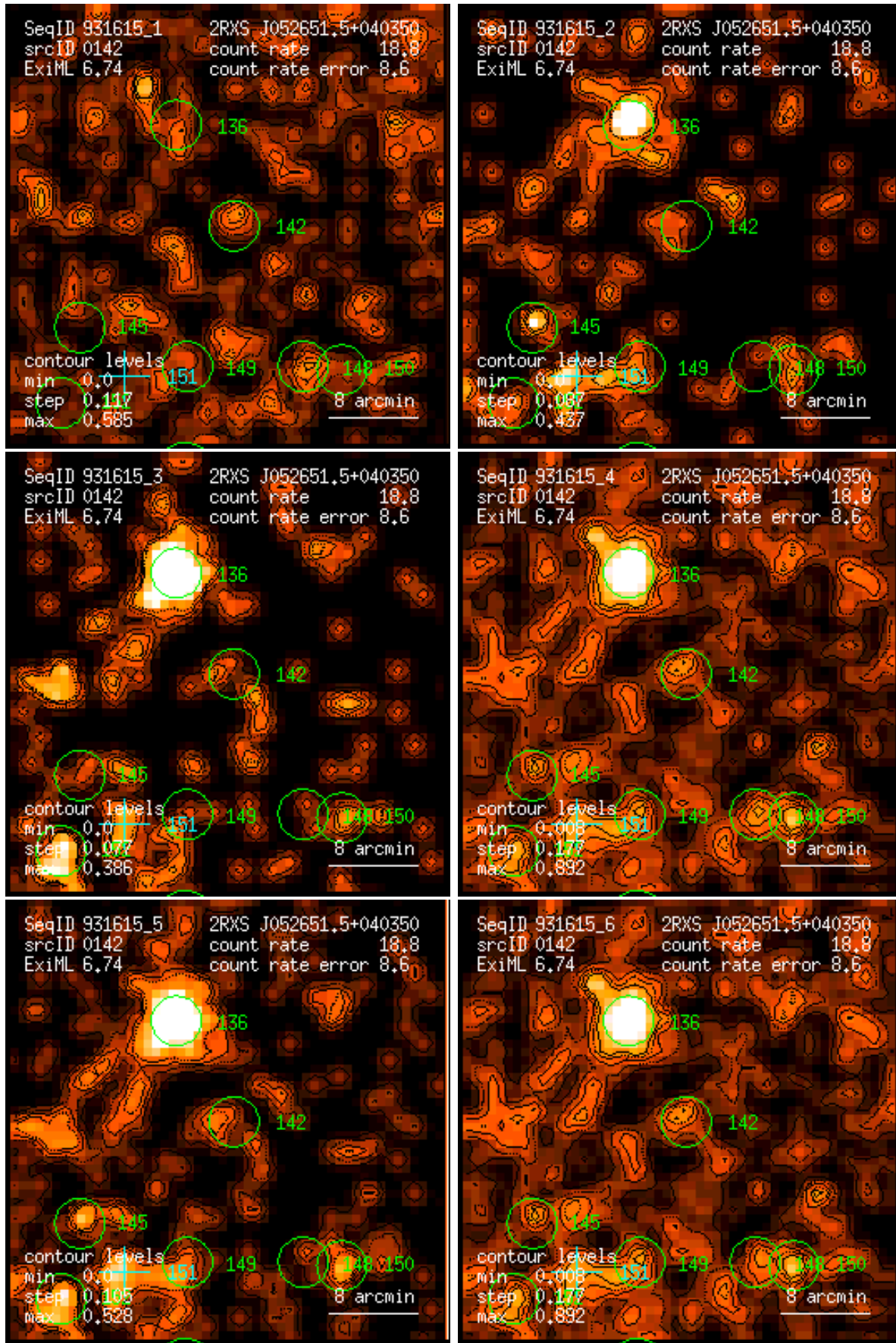
Figure 142: RASS 931615: detection 0142: band rate images, Gaussian filter: (1) PSPC channels 11 – 41, (2) 52 – 90, (3) 91 – 201, (4) 11 – 235, (5) 52 – 201, (6) 11 – 201. Broad band rates in counts/ks. Band rate contour levels in counts/ks/arcmin 2 .
