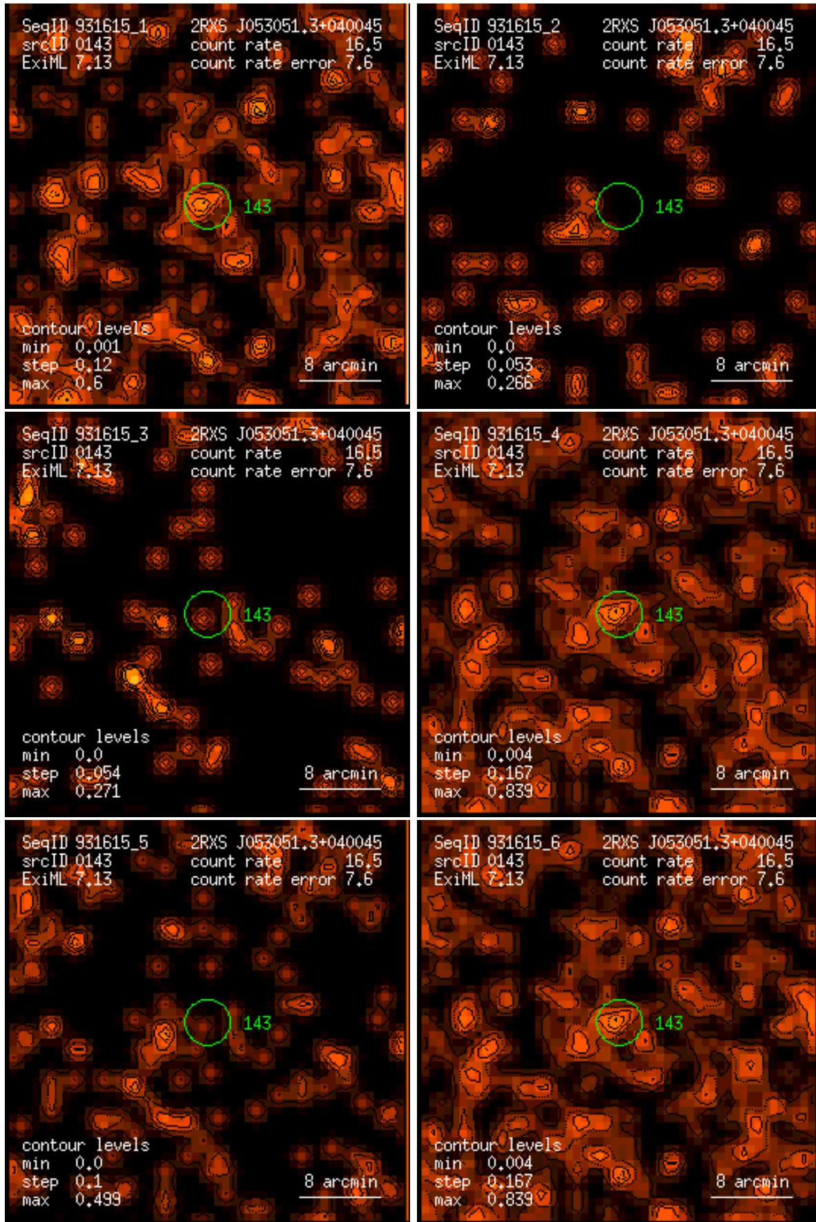
Figure 143: RASS 931615: detection 0143: band rate images, Gaussian filter: (1) PSPC channels 11 – 41, (2) 52 – 90, (3) 91 – 201, (4) 11 – 235, (5) 52 – 201, (6) 11 – 201. Broad band rates in counts/ks. Band rate contour levels in counts/ks/arcmin 2 .
