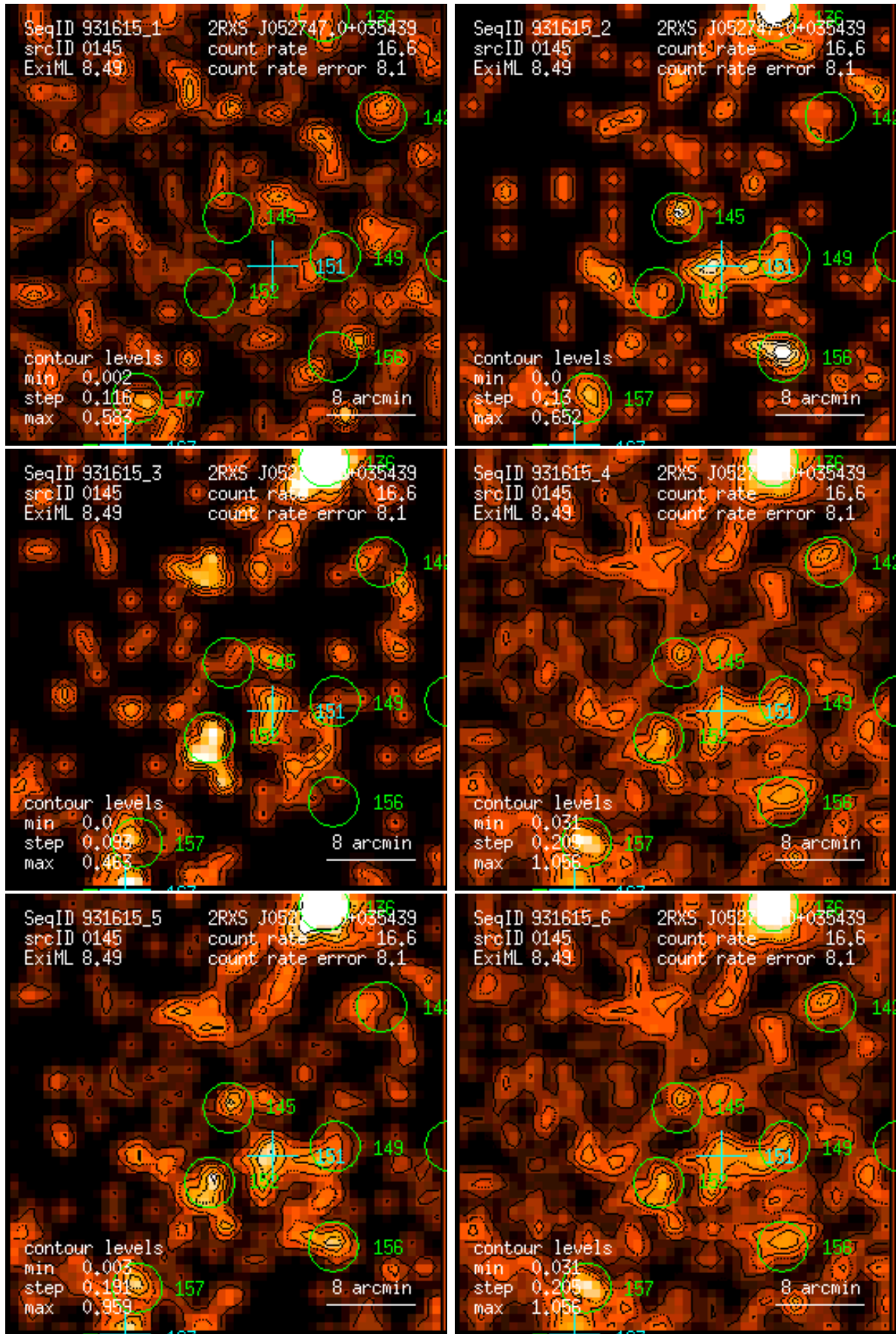
Figure 145: RASS 931615: detection 0145: band rate images, Gaussian filter: (1) PSPC channels 11 – 41, (2) 52 – 90, (3) 91 – 201, (4) 11 – 235, (5) 52 – 201, (6) 11 – 201. Broad band rates in counts/ks. Band rate contour levels in counts/ks/arcmin 2 .
