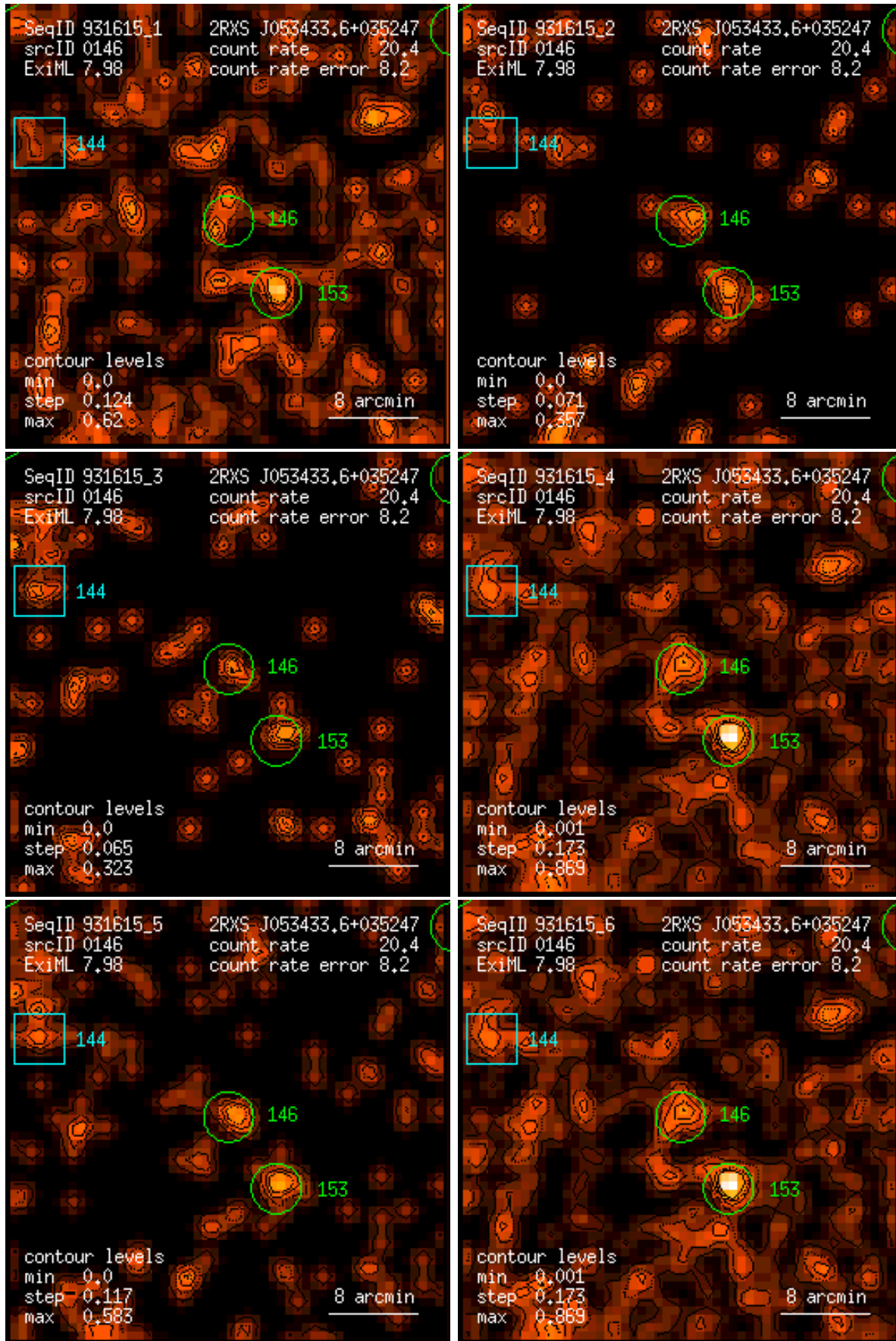
Figure 146: RASS 931615: detection 0146: band rate images, Gaussian filter: (1) PSPC channels 11 – 41, (2) 52 – 90, (3) 91 – 201, (4) 11 – 235, (5) 52 – 201, (6) 11 – 201. Broad band rates in counts/ks. Band rate contour levels in counts/ks/arcmin 2 .
