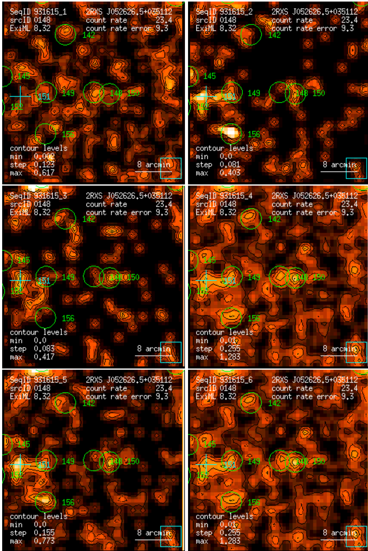
Figure 148: RASS 931615: detection 0148: band rate images, Gaussian filter: (1) PSPC channels 11 – 41, (2) 52 – 90, (3) 91 – 201, (4) 11 – 235, (5) 52 – 201, (6) 11 – 201. Broad band rates in counts/ks. Band rate contour levels in counts/ks/arcmin 2 .
