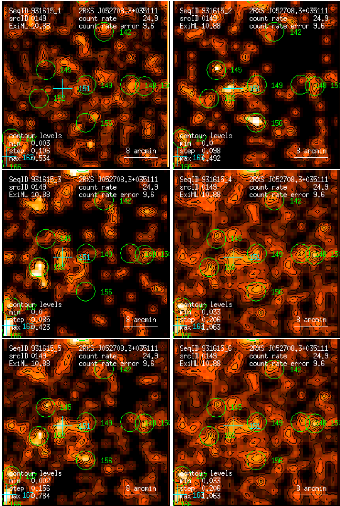
Figure 149: RASS 931615: detection 0149: band rate images, Gaussian filter: (1) PSPC channels 11 – 41, (2) 52 – 90, (3) 91 – 201, (4) 11 – 235, (5) 52 – 201, (6) 11 – 201. Broad band rates in counts/ks. Band rate contour levels in counts/ks/arcmin 2 .
