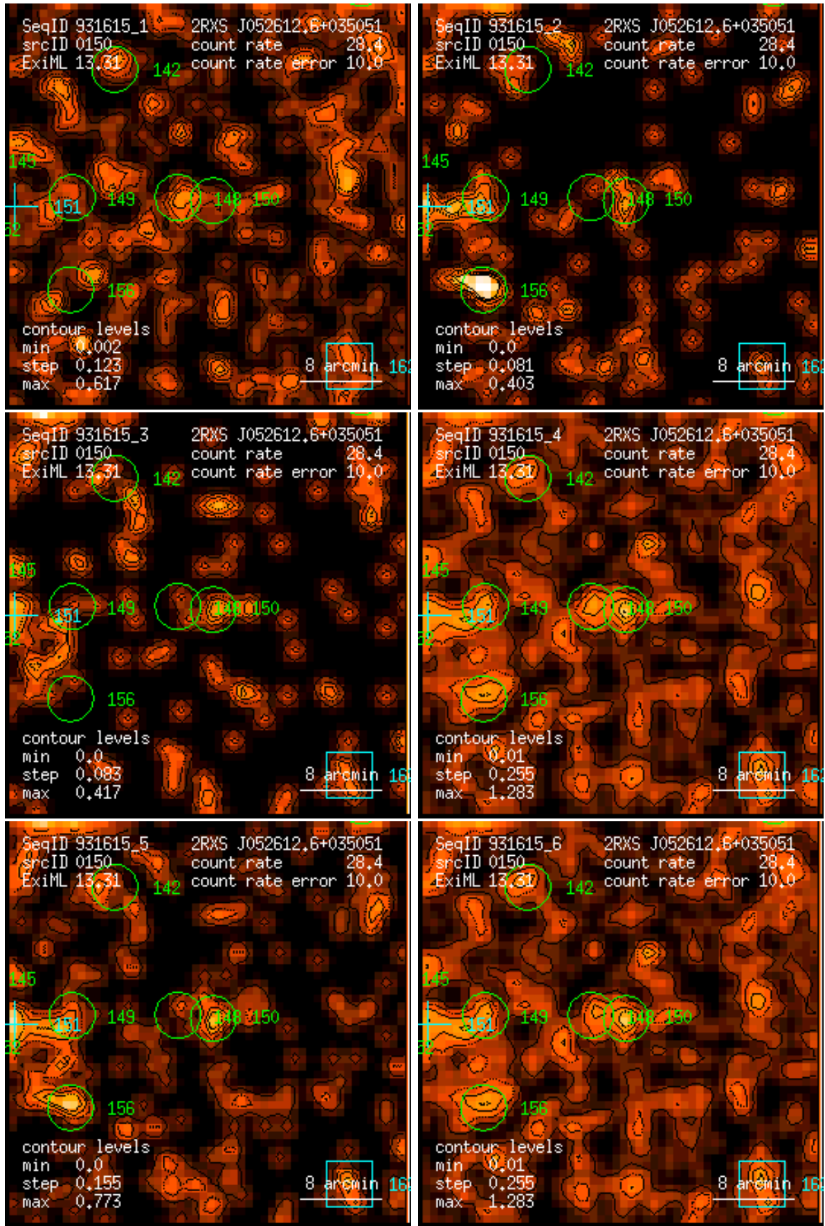
Figure 150: RASS 931615: detection 0150: band rate images, Gaussian filter: (1) PSPC channels 11 – 41, (2) 52 – 90, (3) 91 – 201, (4) 11 – 235, (5) 52 – 201, (6) 11 – 201. Broad band rates in counts/ks. Band rate contour levels in counts/ks/arcmin 2 .
