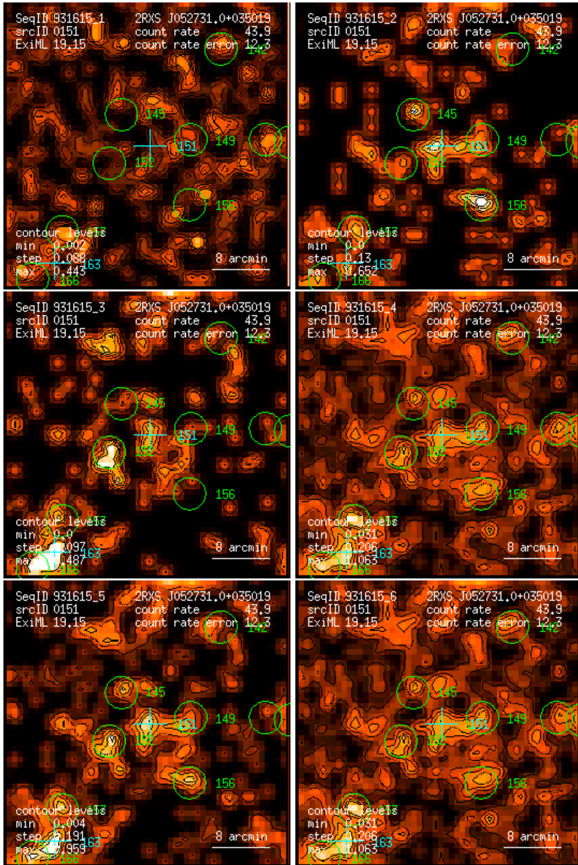
Figure 151: RASS 931615: detection 0151: band rate images, Gaussian filter: (1) PSPC channels 11 – 41, (2) 52 – 90, (3) 91 – 201, (4) 11 – 235, (5) 52 – 201, (6) 11 – 201. Broad band rates in counts/ks. Band rate contour levels in counts/ks/arcmin 2 .
