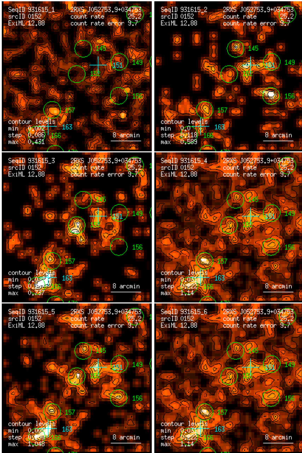
Figure 152: RASS 931615: detection 0152: band rate images, Gaussian filter: (1) PSPC channels 11 – 41, (2) 52 – 90, (3) 91 – 201, (4) 11 – 235, (5) 52 – 201, (6) 11 – 201. Broad band rates in counts/ks. Band rate contour levels in counts/ks/arcmin 2 .
