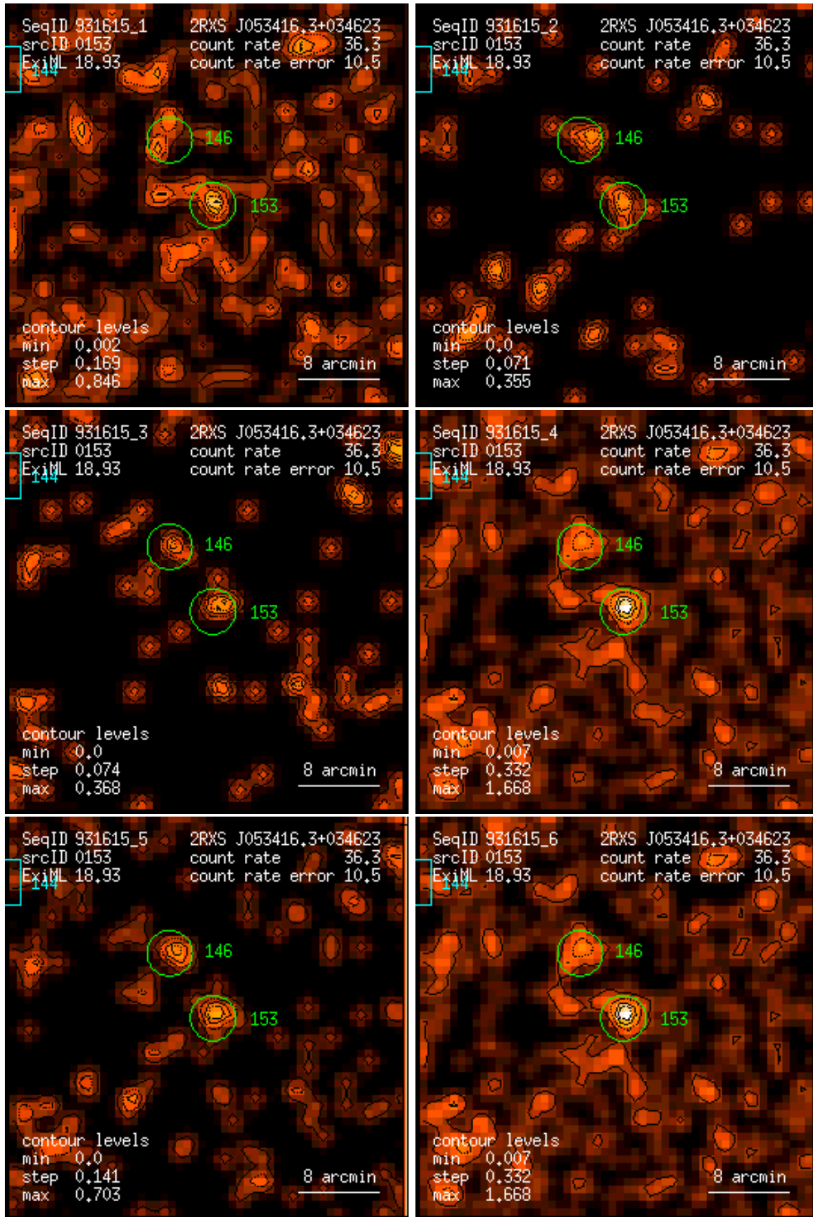
Figure 153: RASS 931615: detection 0153: band rate images, Gaussian filter: (1) PSPC channels 11 – 41, (2) 52 – 90, (3) 91 – 201, (4) 11 – 235, (5) 52 – 201, (6) 11 – 201. Broad band rates in counts/ks. Band rate contour levels in counts/ks/arcmin 2 .
