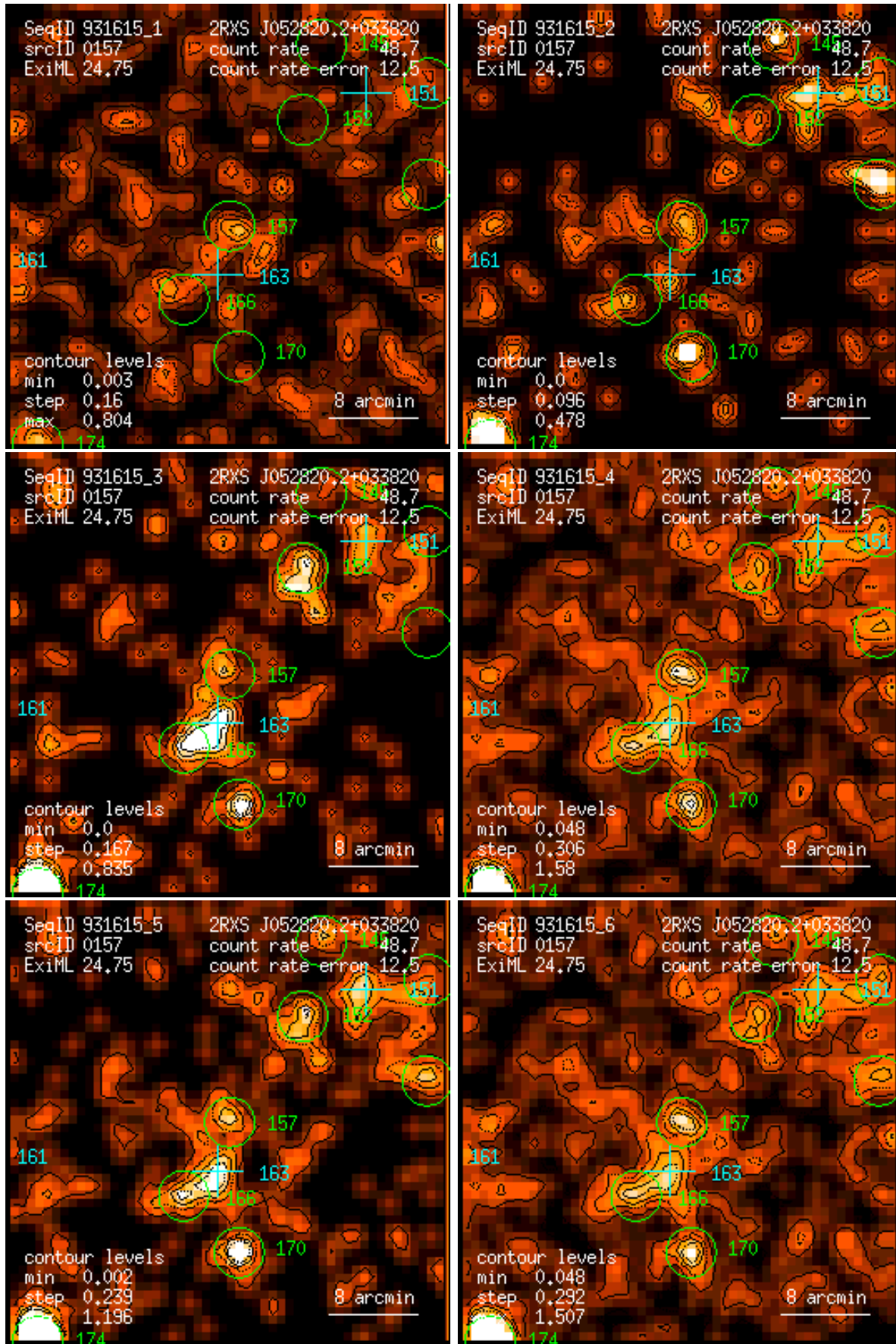
Figure 157: RASS 931615: detection 0157: band rate images, Gaussian filter: (1) PSPC channels 11 – 41, (2) 52 – 90, (3) 91 – 201, (4) 11 – 235, (5) 52 – 201, (6) 11 – 201. Broad band rates in counts/ks. Band rate contour levels in counts/ks/arcmin 2 .
