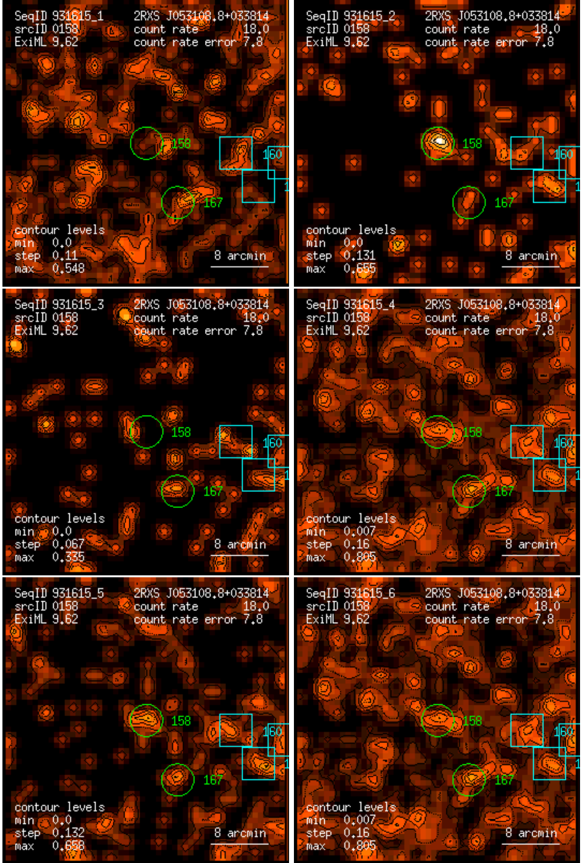
Figure 158: RASS 931615: detection 0158: band rate images, Gaussian filter: (1) PSPC channels 11 – 41, (2) 52 – 90, (3) 91 – 201, (4) 11 – 235, (5) 52 – 201, (6) 11 – 201. Broad band rates in counts/ks. Band rate contour levels in counts/ks/arcmin 2 .
