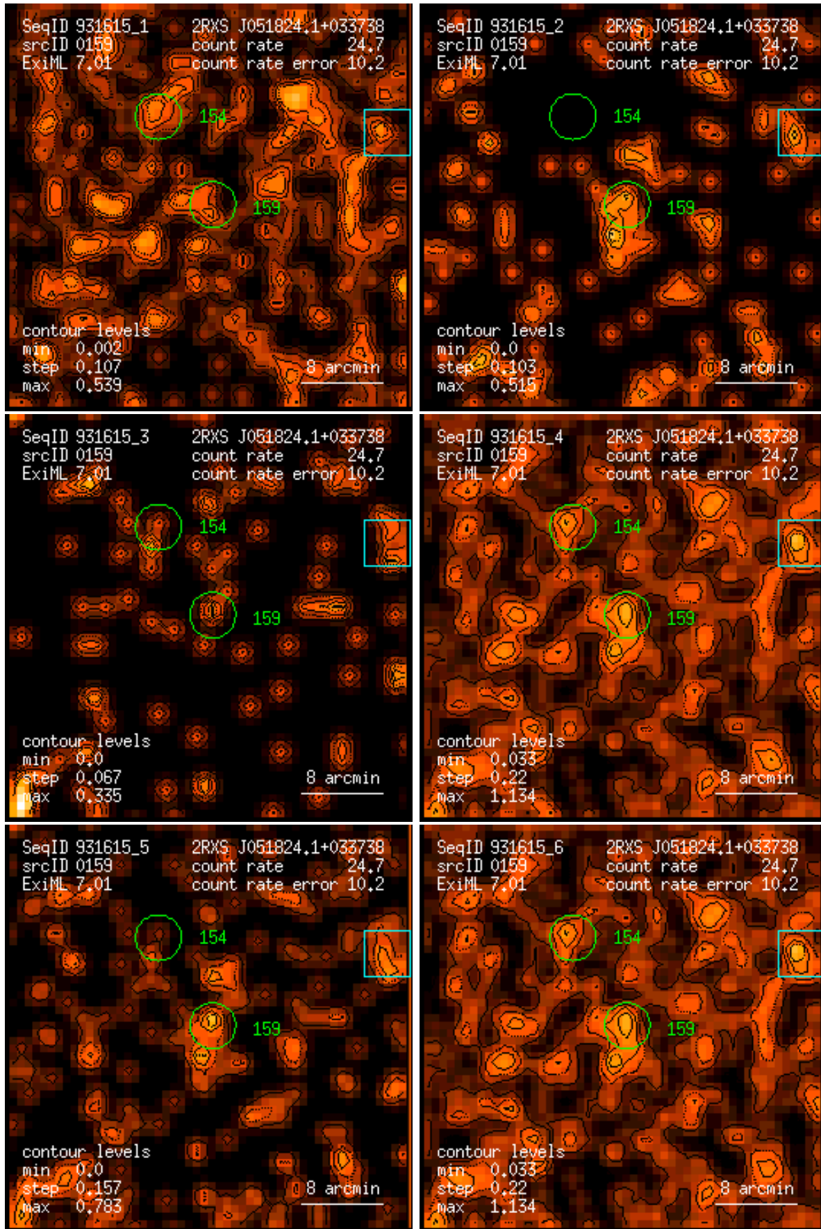
Figure 159: RASS 931615: detection 0159: band rate images, Gaussian filter: (1) PSPC channels 11 – 41, (2) 52 – 90, (3) 91 – 201, (4) 11 – 235, (5) 52 – 201, (6) 11 – 201. Broad band rates in counts/ks. Band rate contour levels in counts/ks/arcmin 2 .
