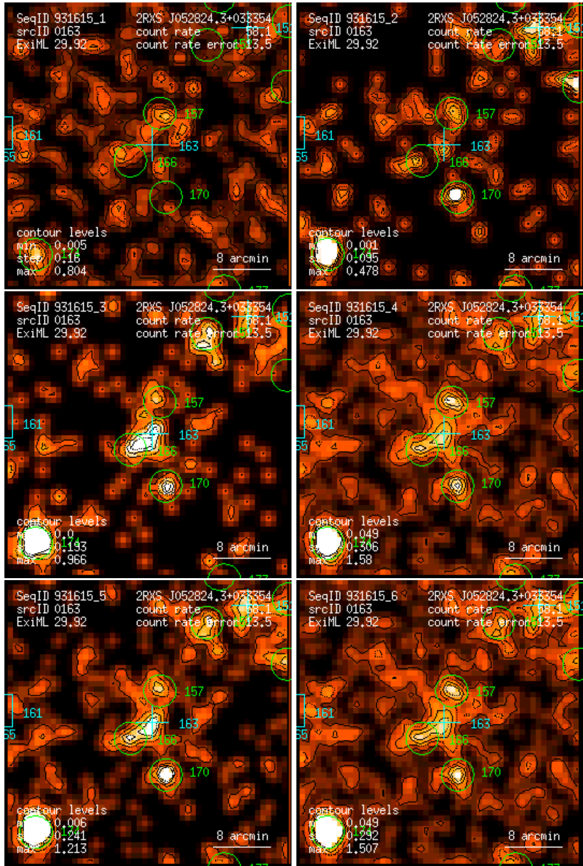
Figure 163: RASS 931615: detection 0163: band rate images, Gaussian filter: (1) PSPC channels 11 – 41, (2) 52 – 90, (3) 91 – 201, (4) 11 – 235, (5) 52 – 201, (6) 11 – 201. Broad band rates in counts/ks. Band rate contour levels in counts/ks/arcmin 2 .
