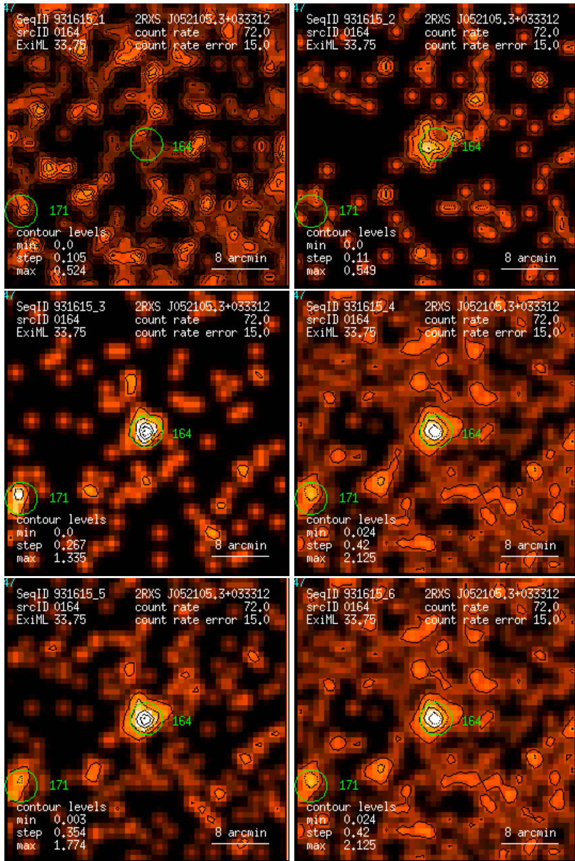
Figure 164: RASS 931615: detection 0164: band rate images, Gaussian filter: (1) PSPC channels 11 – 41, (2) 52 – 90, (3) 91 – 201, (4) 11 – 235, (5) 52 – 201, (6) 11 – 201. Broad band rates in counts/ks. Band rate contour levels in counts/ks/arcmin 2 .
