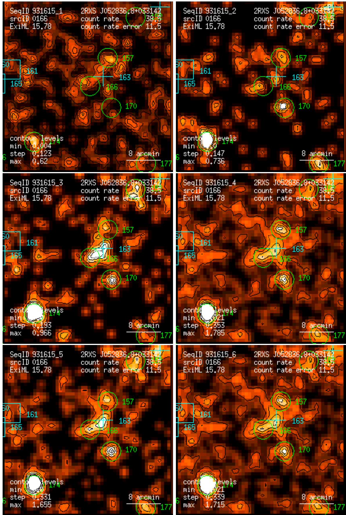
Figure 166: RASS 931615: detection 0166: band rate images, Gaussian filter: (1) PSPC channels 11 – 41, (2) 52 – 90, (3) 91 – 201, (4) 11 – 235, (5) 52 – 201, (6) 11 – 201. Broad band rates in counts/ks. Band rate contour levels in counts/ks/arcmin 2 .
