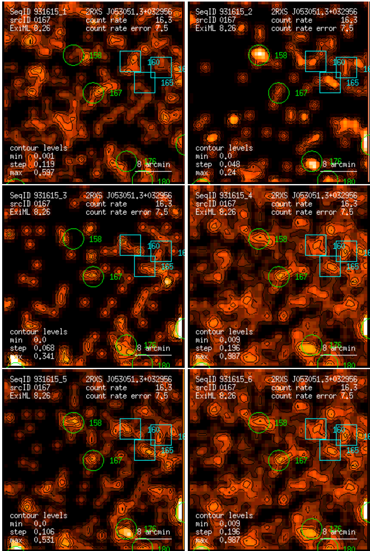
Figure 167: RASS 931615: detection 0167: band rate images, Gaussian filter: (1) PSPC channels 11 – 41, (2) 52 – 90, (3) 91 – 201, (4) 11 – 235, (5) 52 – 201, (6) 11 – 201. Broad band rates in counts/ks. Band rate contour levels in counts/ks/arcmin 2 .
