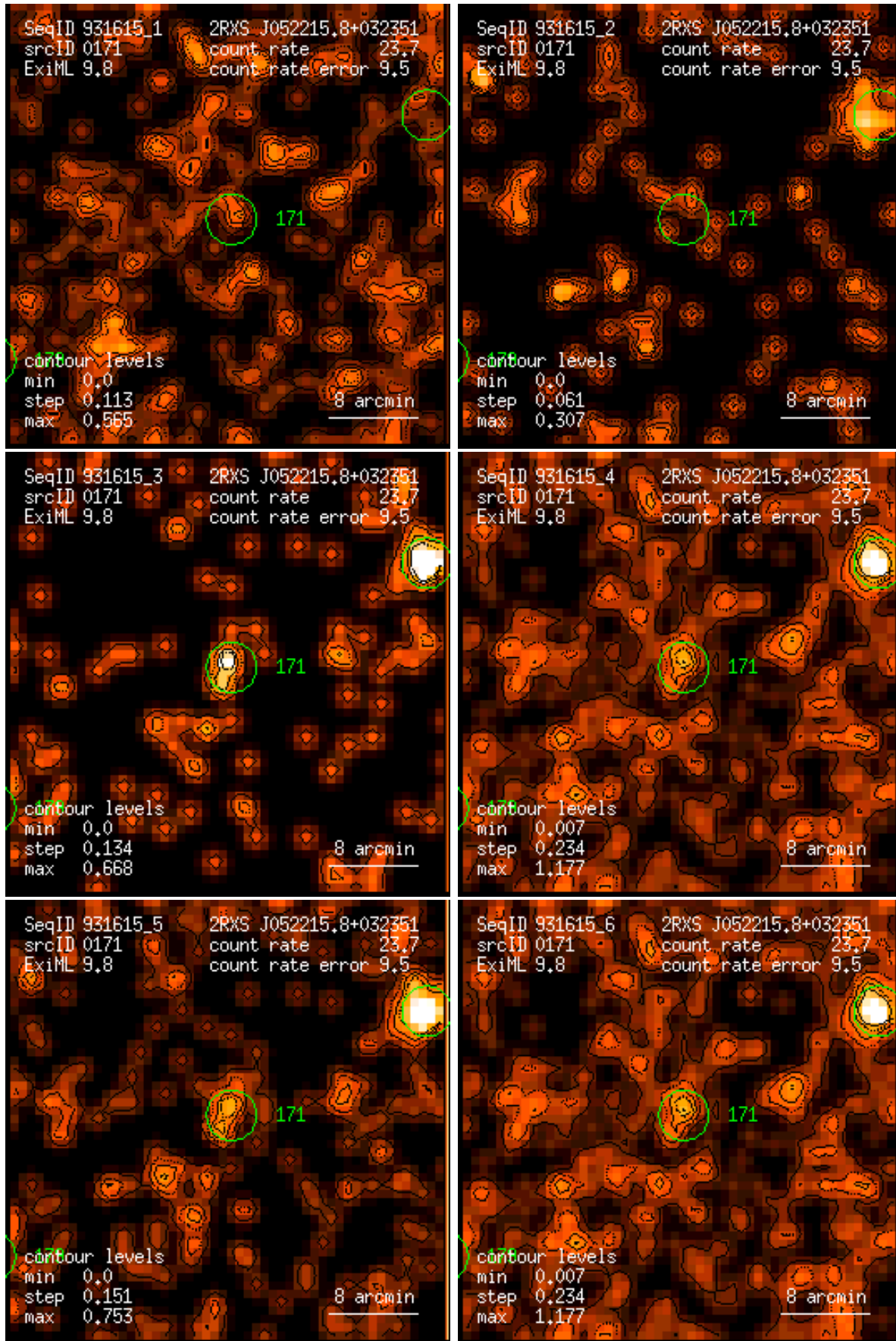
Figure 171: RASS 931615: detection 0171: band rate images, Gaussian filter: (1) PSPC channels 11 – 41, (2) 52 – 90, (3) 91 – 201, (4) 11 – 235, (5) 52 – 201, (6) 11 – 201. Broad band rates in counts/ks. Band rate contour levels in counts/ks/arcmin 2 .
