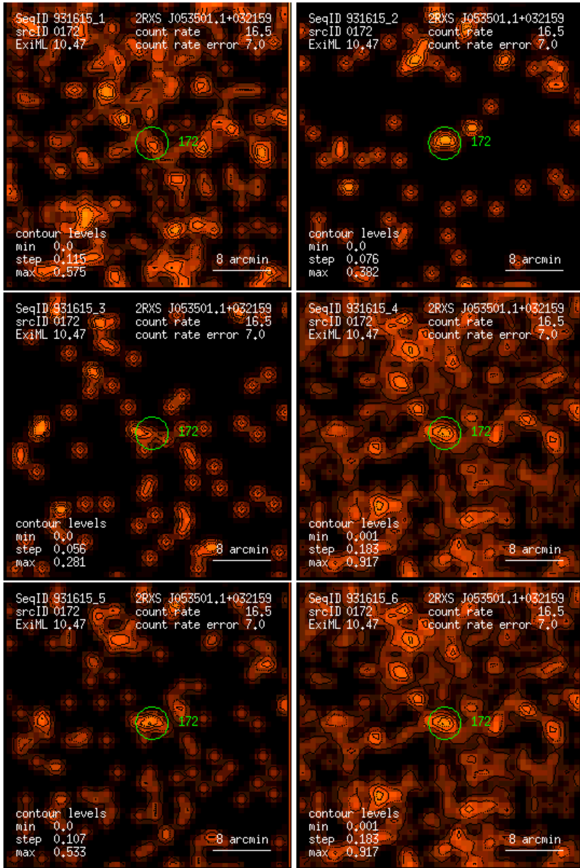
Figure 172: RASS 931615: detection 0172: band rate images, Gaussian filter: (1) PSPC channels 11 – 41, (2) 52 – 90, (3) 91 – 201, (4) 11 – 235, (5) 52 – 201, (6) 11 – 201. Broad band rates in counts/ks. Band rate contour levels in counts/ks/arcmin 2 .
